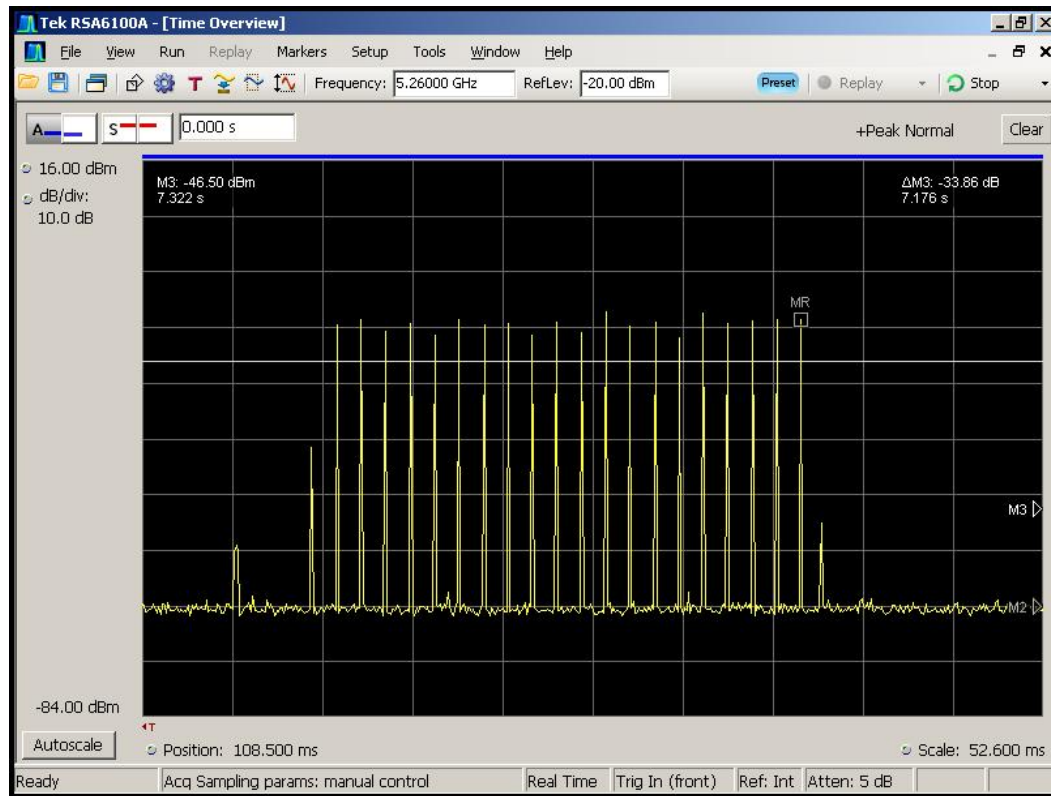
Figure 5-1. Type 1 Radar Pulse
