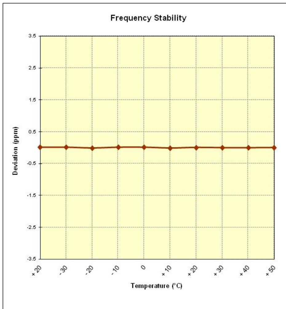
Figure 6-6. Frequency Stability Graph (Band 4)
