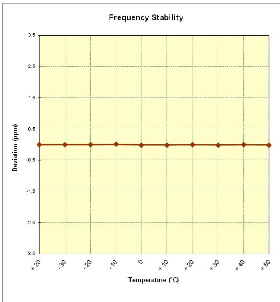
Figure 6-7. Frequency Stability Graph (Band 2)
