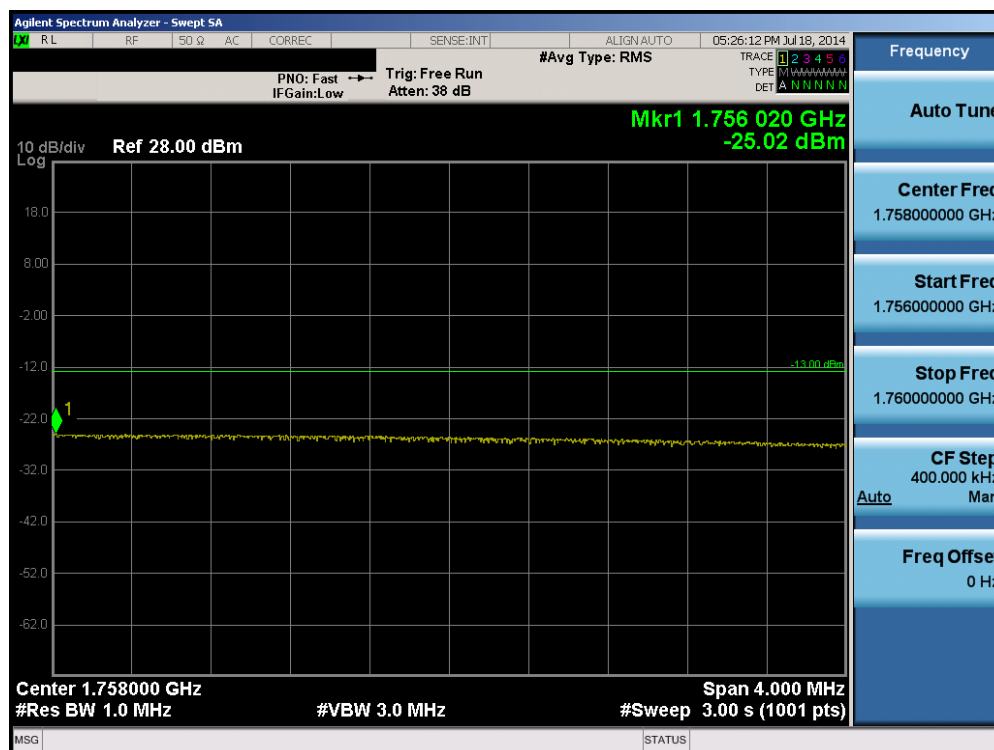
Plot 6-24. Upper Extended Band Edge Plot (Band 4 – 15.0MHz QPSK – RB Size 75)
