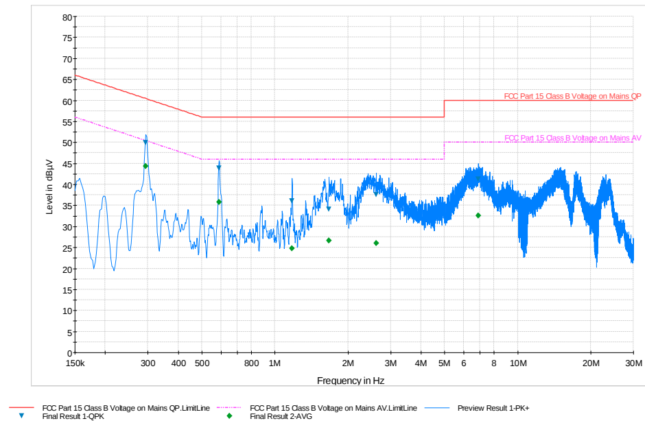
Plot 6-20. Line Conducted Plot with ANT+ (L1)
