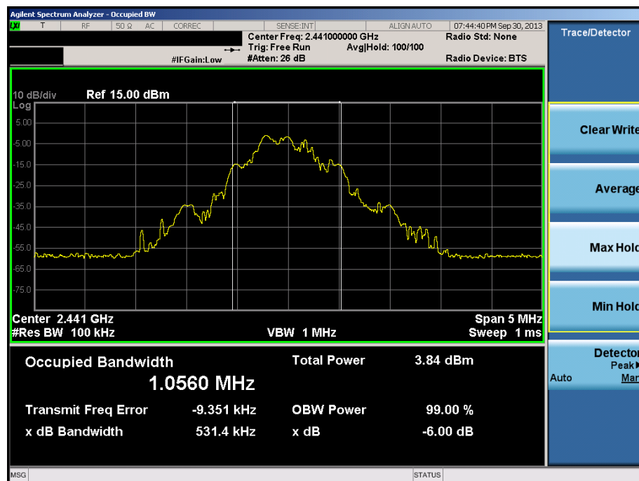
Plot 6-2. 6dB Bandwidth Plot (2441MHz – Mid Channel)
