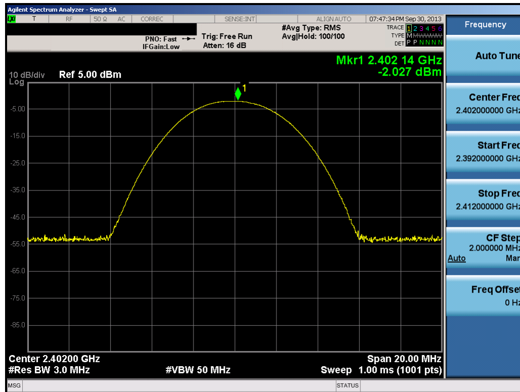
Plot 6-5. Peak Power Plot (2402MHz – Low Channel)
