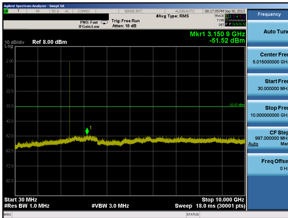
Plot 6-12. Conducted Spurious Plot (2402MHz – Low Channel)
