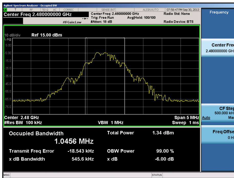
Plot 6-3. 6dB Bandwidth Plot (2480MHz – High Channel)
