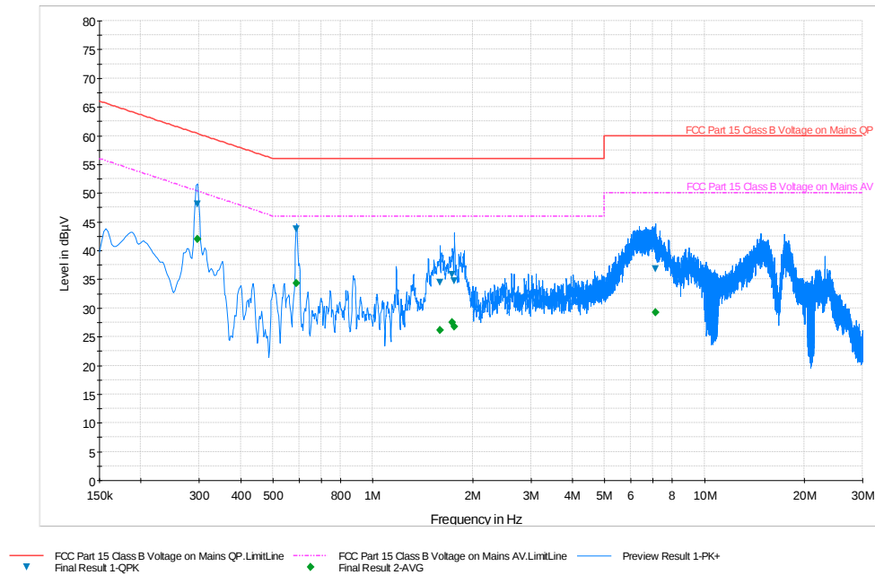
Plot 6-21. Line Conducted Plot with ANT+ (N)
