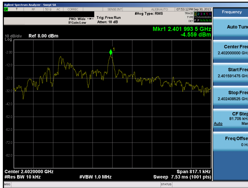
Plot 6-7. Power Spectral Density Plot (2402MHz – Low Channel)
