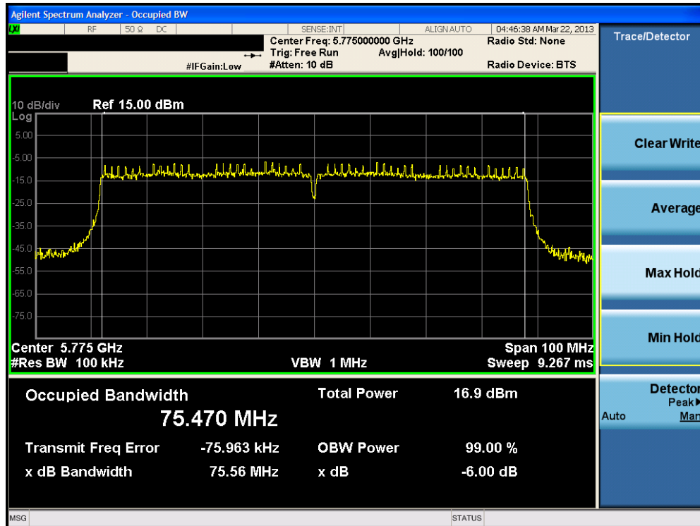
Plot 6-18. 6dB Bandwidth Plot (80MHz BW 802.11n (5.8GHz) – Ch. 155)
