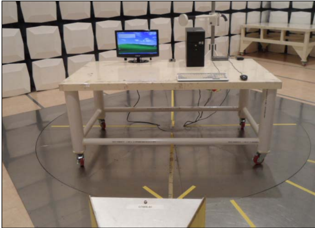
[ Radiated Disturbance for Above 1 GHz – Front ]
