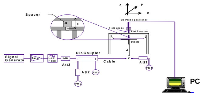
Figure 7.1 Dipole Validation Test Setup
