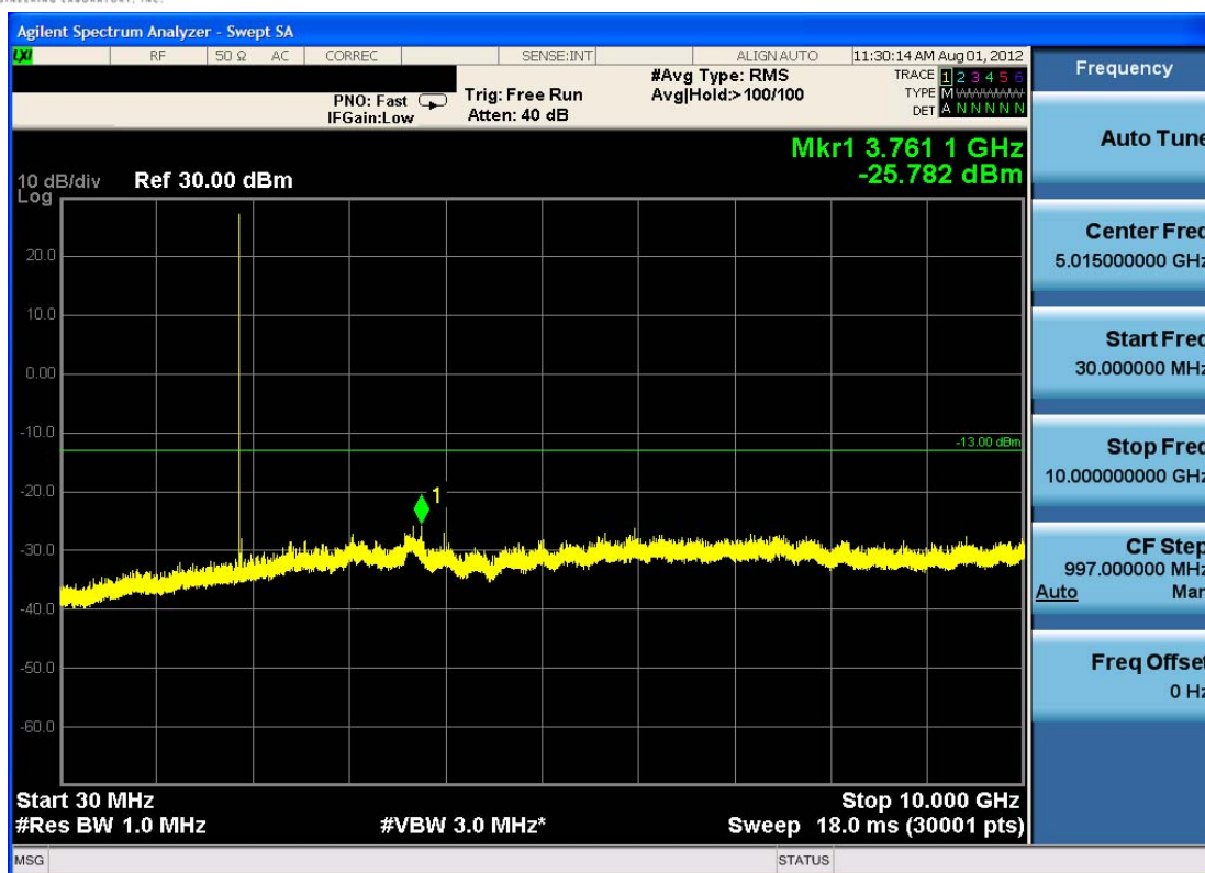
Plot 7-5. Conducted Spurious Plot (PCS CDMA Mode – Ch. 600)
