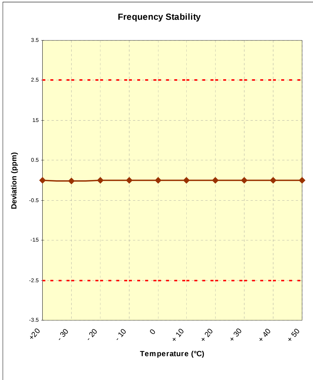
Figure 6-1. Frequency Stability Graph (PCS CDMA Mode – Ch. 600)
