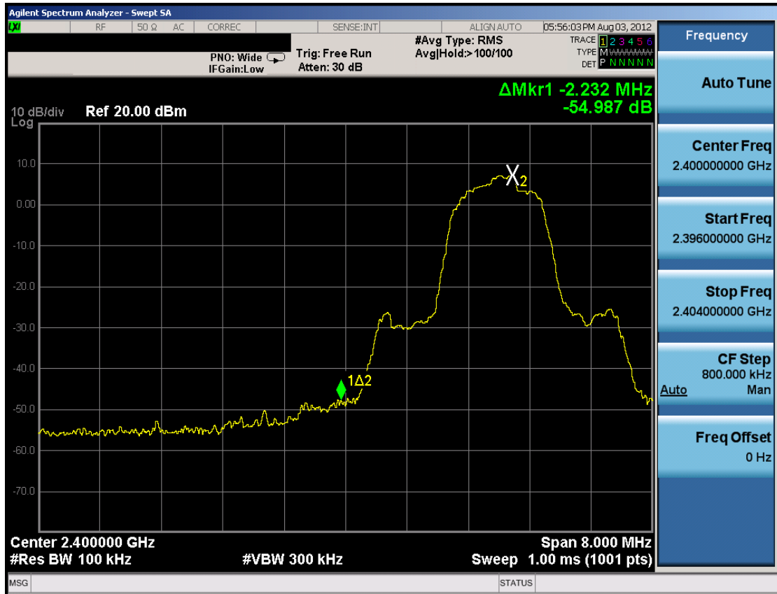
Plot 6-19. Band Edge Plot (Bluetooth with Hopping Disabled, 3Mbps – Ch. 0)
