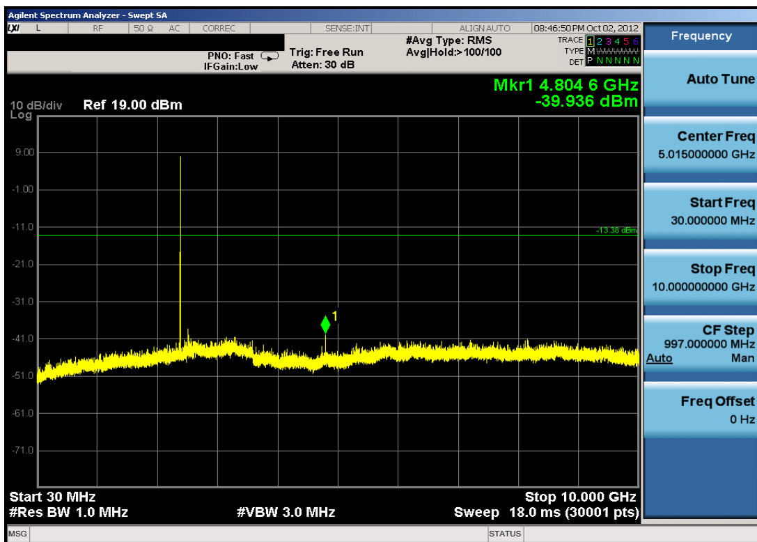
Plot 6-27. Conducted Spurious Plot (Bluetooth, 3Mbps – Ch. 0)
