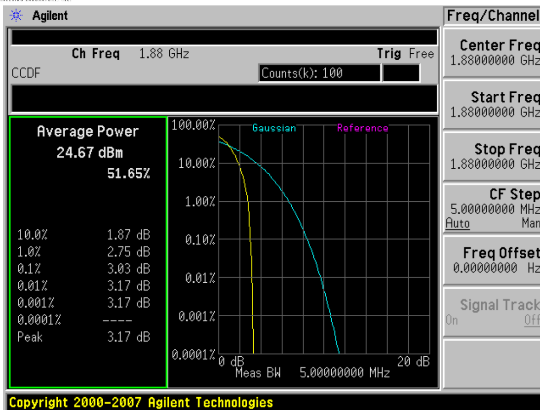
Plot 7-19. Peak-Average Ratio Plot (PCS CDMA Mode – Ch. 600)
