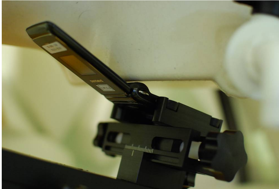
Figure 18-1 SAR Test Setup Photo 1
