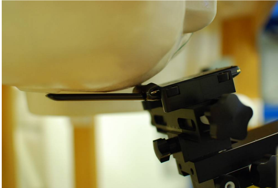
Figure 18-3 SAR Test Setup Photo 3
