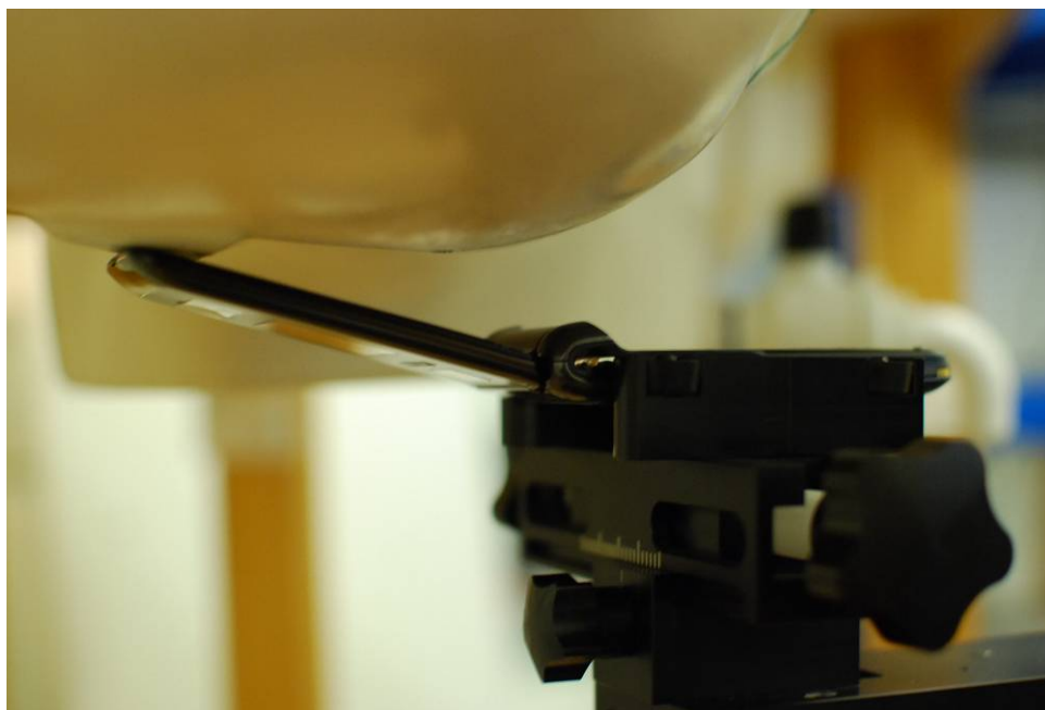
Figure 18-4 SAR Test Setup Photo 4
