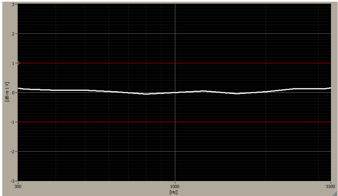
Figure 6-3 Helmholtz Coil Validation for Frequency Response
