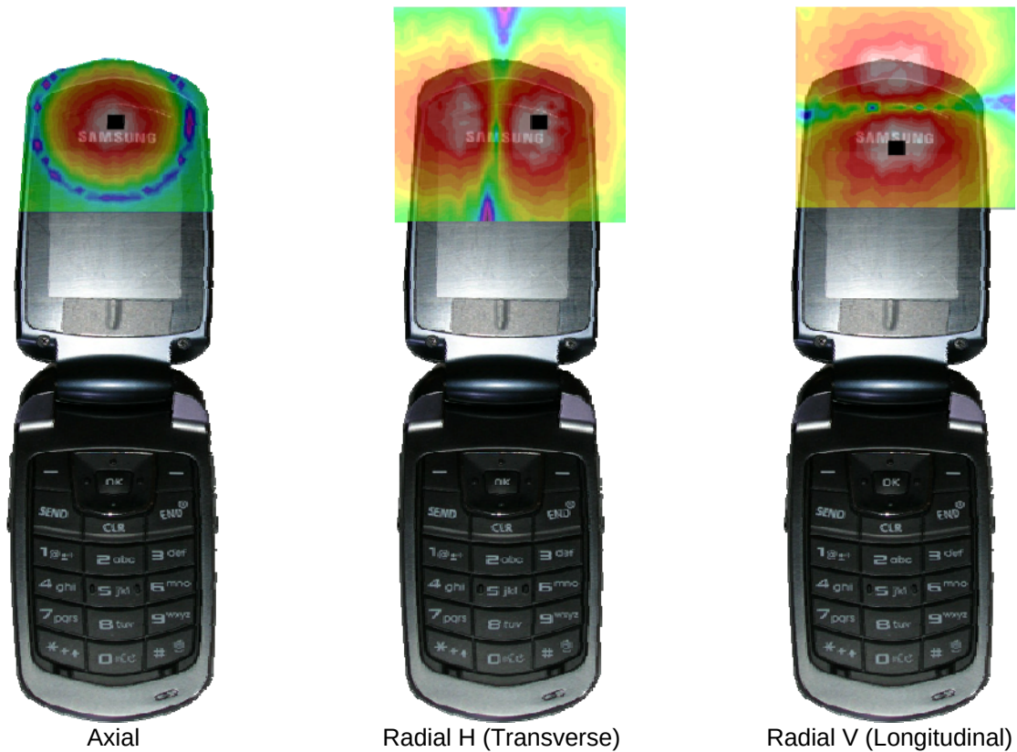
Figure 13-3 T-Coil Scan Overlay Magnetic Field Distributions
