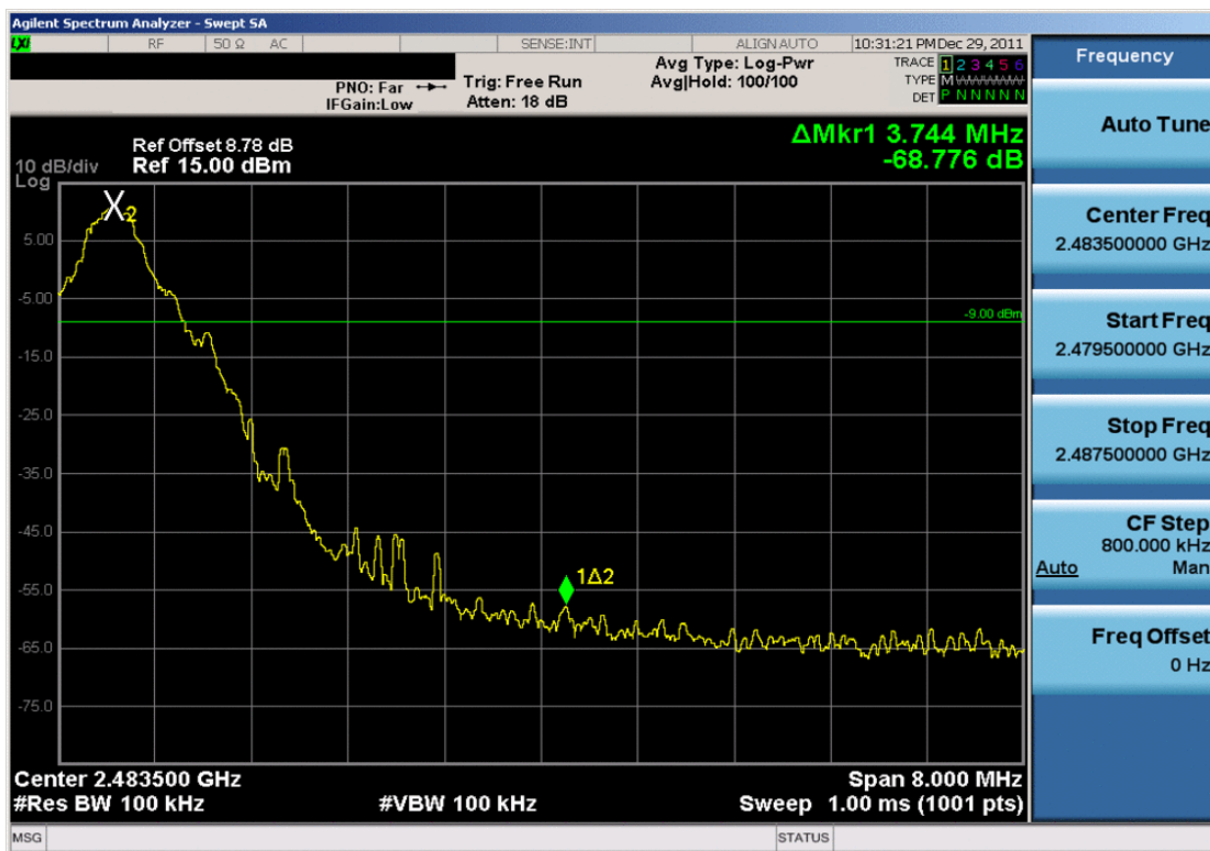
Plot 6-11. Band Edge Plot, Hopping Stopped (Bluetooth, 1Mbps – Ch. 78)
