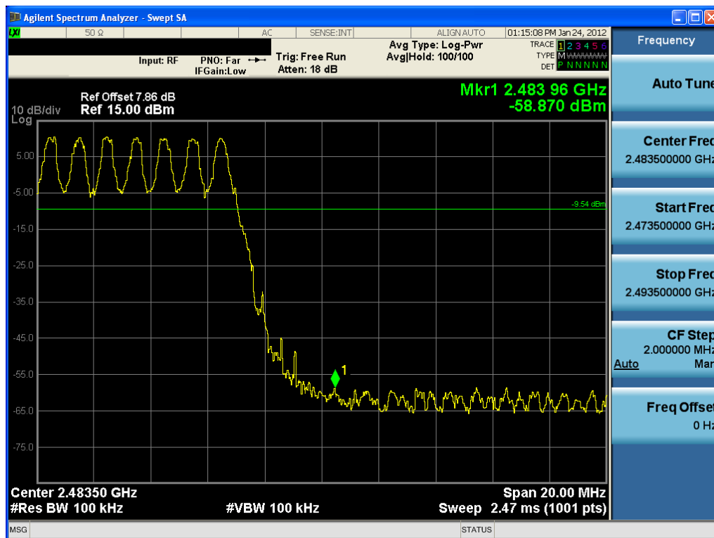
Plot 6-13. Band Edge Plot, Hopping Enabled (Bluetooth, 1Mbps – Ch. 78)
