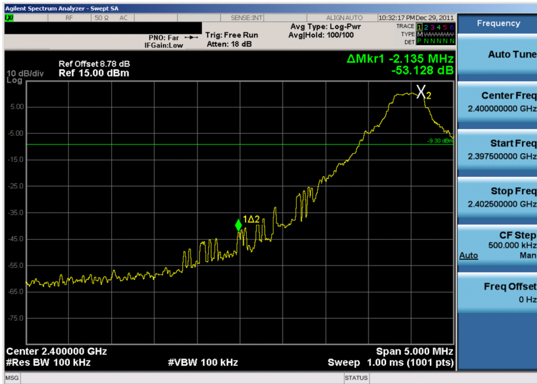
Plot 6-10. Band Edge Plot, Hopping Stopped (Bluetooth, 1Mbps – Ch. 0)
