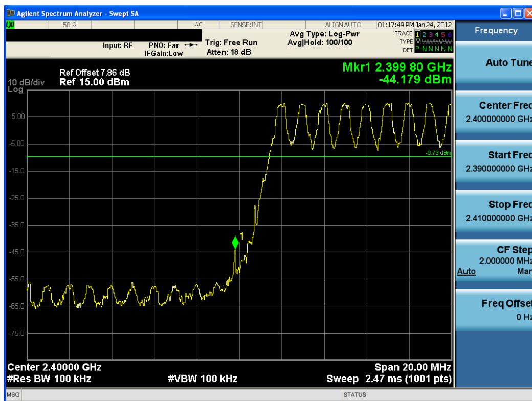
Plot 6-12. Band Edge Plot, Hopping Enabled (Bluetooth, 1Mbps – Ch. 0)
