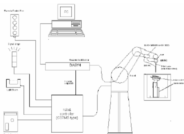
Figure 3.1 HAC Measurement System Setup
