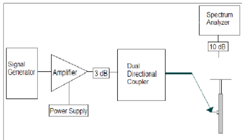
Figure 8.1 Setup to Dipole
