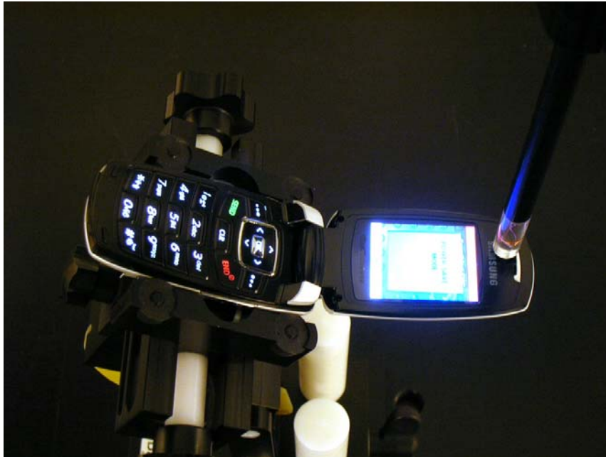
Figure 0-1 Test Setup for Wireless Device
