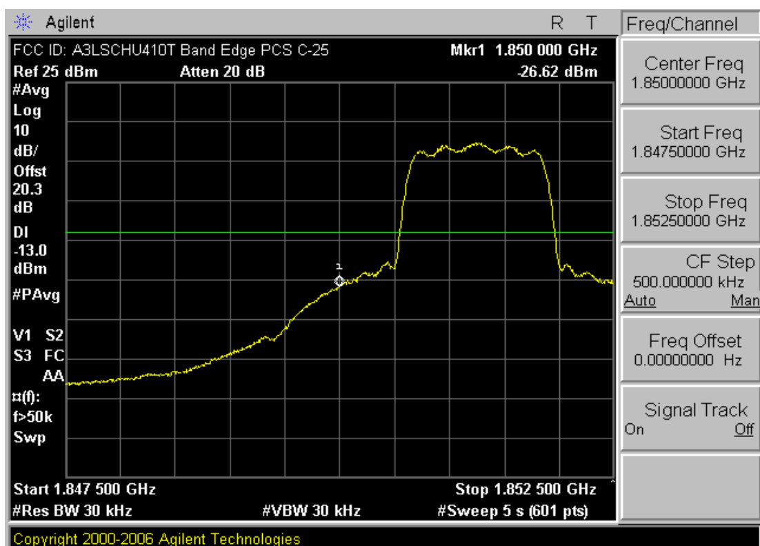
Plot 7-279. Band Edge Plot (PCS CDMA Mode – Ch. 25)
