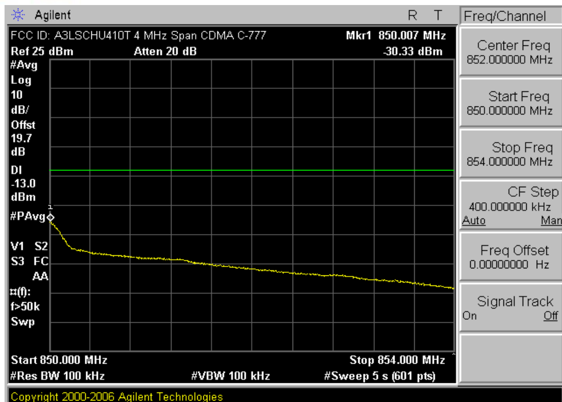
Plot 7-24. 4MHz Span Plot (Cellular CDMA Mode – Ch. 777)
