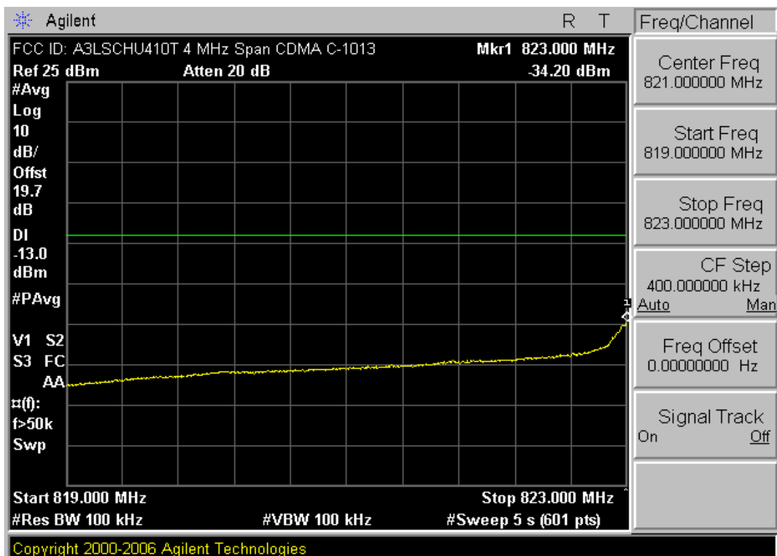
Plot 7-18. 4MHz Span Plot (Cellular CDMA Mode – Ch. 1013)
