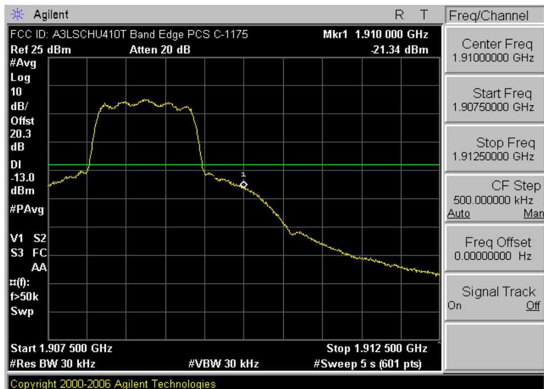
Plot 7-32. Band Edge Plot (PCS CDMA Mode – Ch. 1175)
