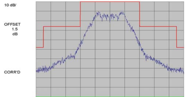
Plot 7-14. SAT + DTMF
