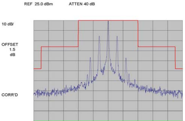
Plot 7-12. Supervisory Audio Tone (SAT)
