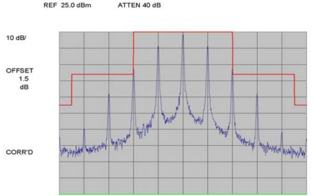
Plot 7-11. Signaling Tone (ST)
