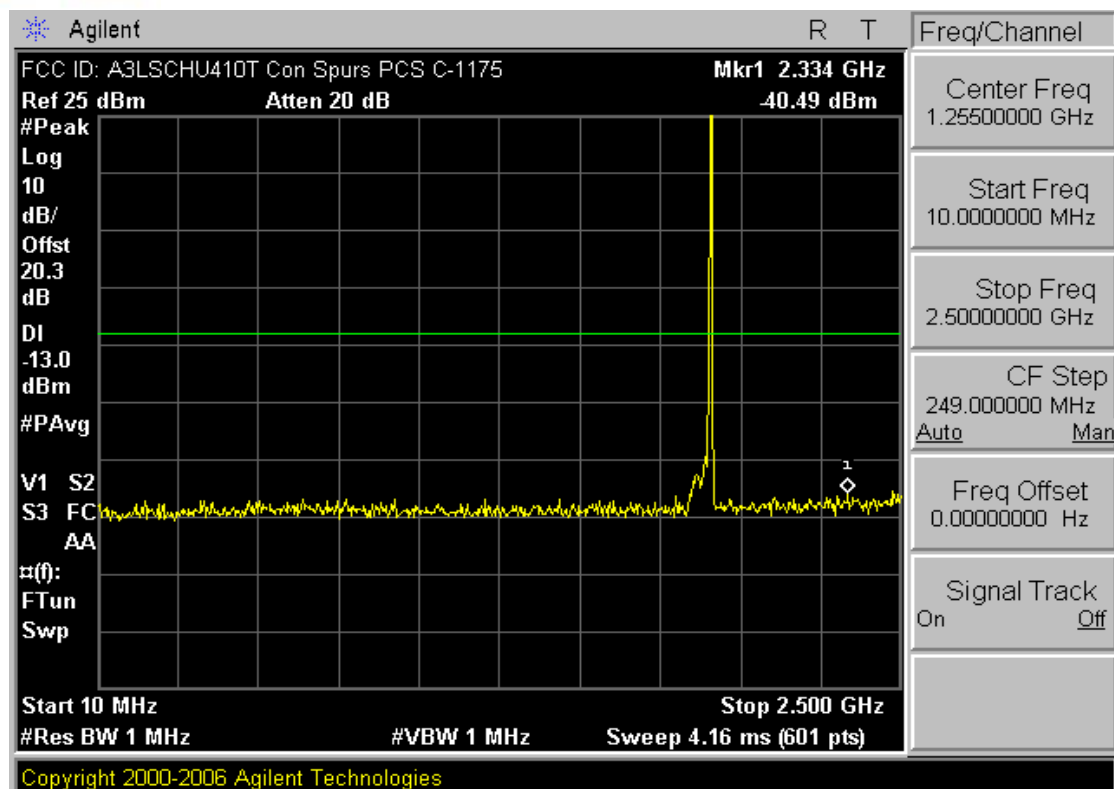
Plot 7-34. Conducted Spurious Plot (PCS CDMA Mode – Ch. 1175)
