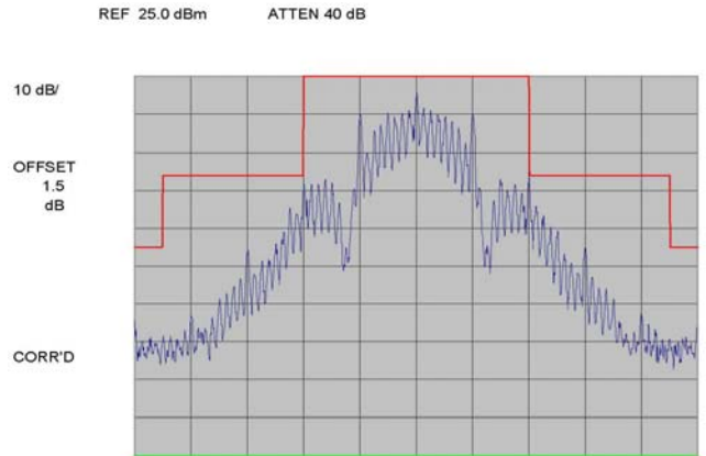
Plot 7-13. Wide Band Data Signal (WBD)
