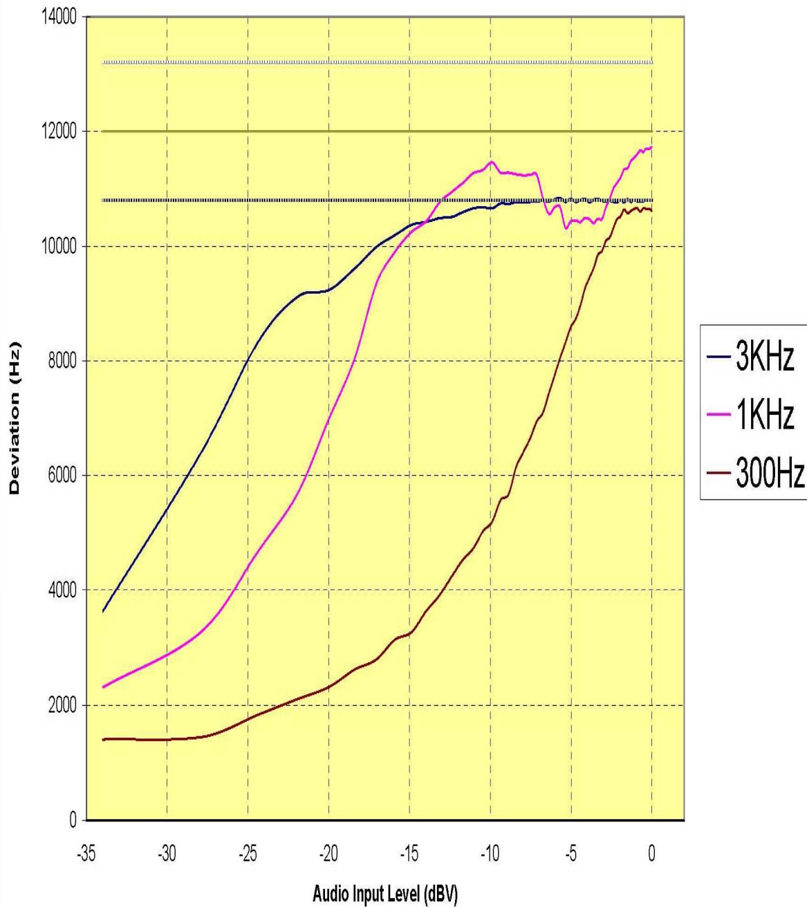
Plot 7-7. Modulation Limiting Plot (AMPS Mode – Ch. 384)
