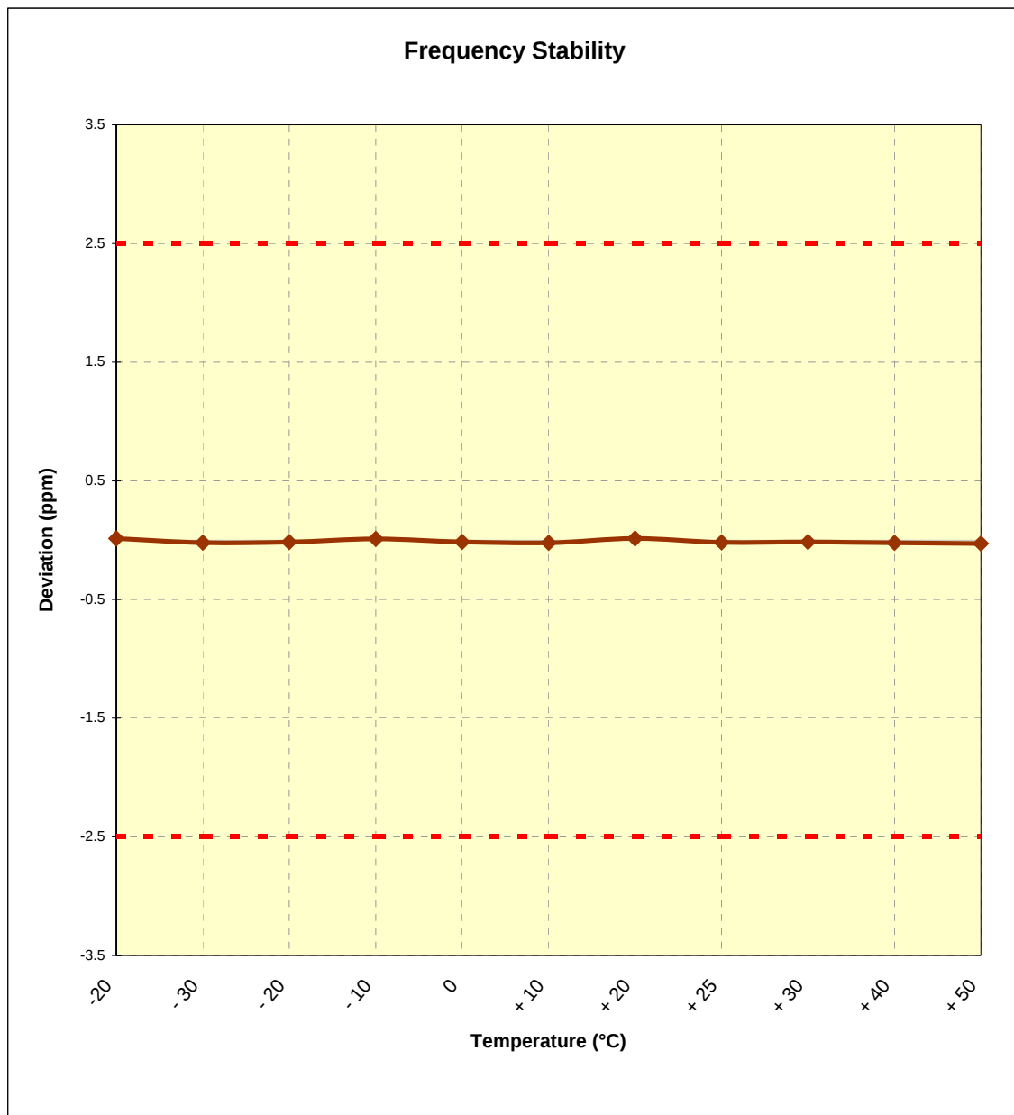
Figure 6-3. Frequency Stability Graph (Cellular CDMA Mode – Ch. 384)
