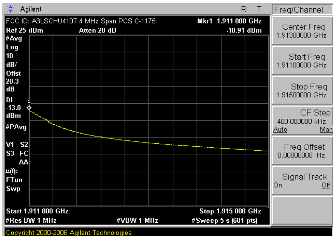
Plot 7-33. 4MHz Span Plot (PCS CDMA Mode – Ch. 1175)
