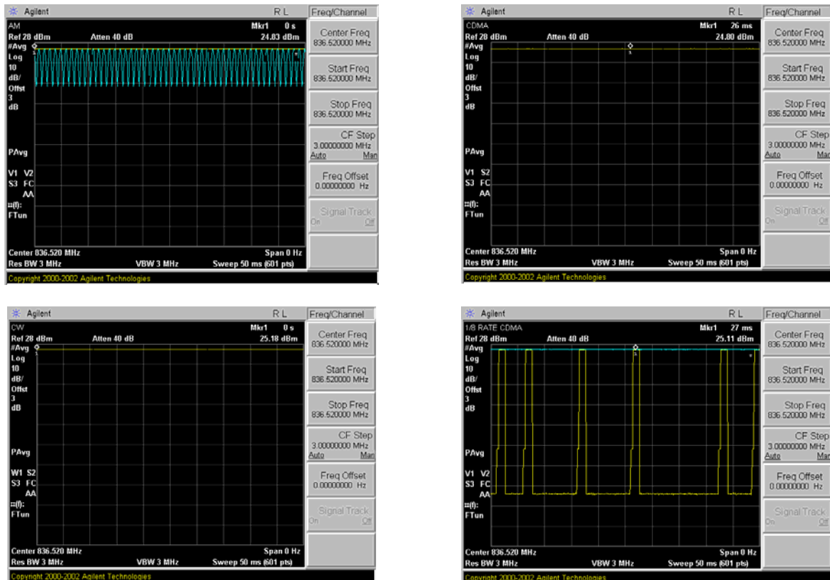
Figure 25 Zero-Span Plots
