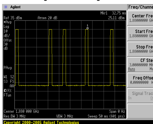
Figure 8.6 1/8 rate Signal
