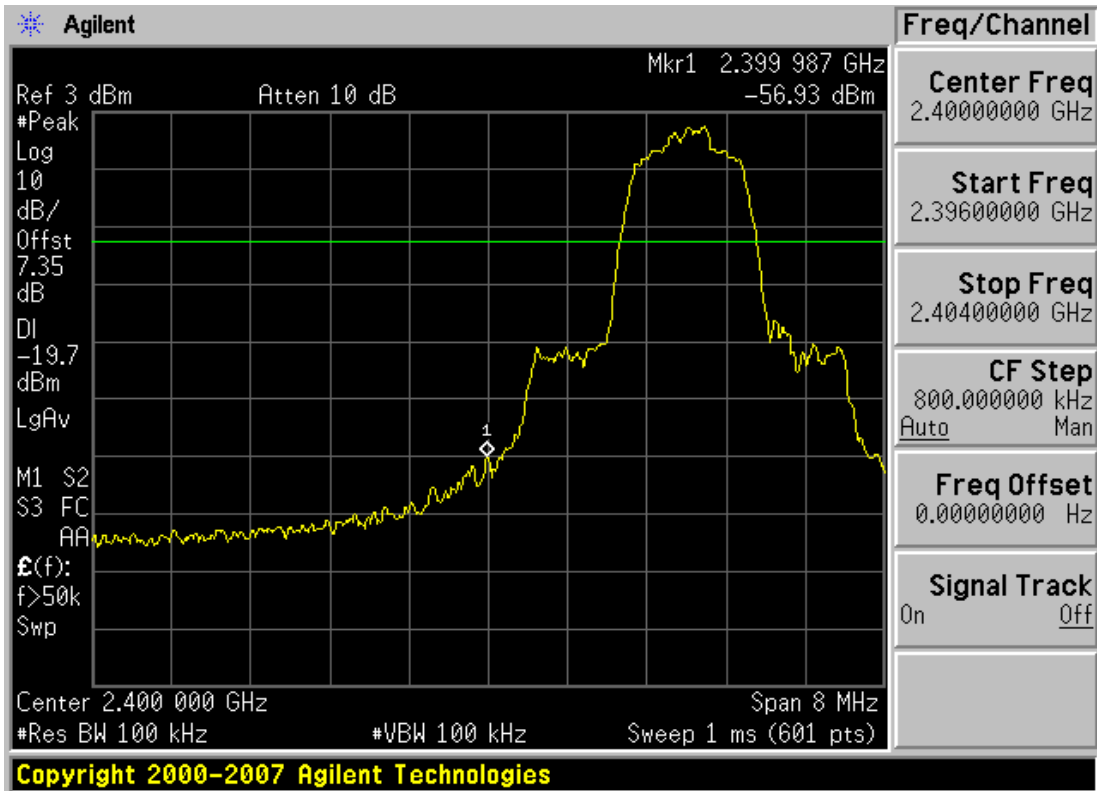
Plot 6-6. Band Edge Plot (Bluetooth 2.1 with Enhanced Data Rates – Ch. 0)
