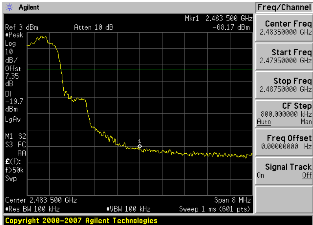
Plot 6-7. Band Edge Plot (Bluetooth 2.1 with Enhanced Data Rates – Ch. 78)
