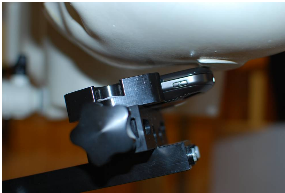
Figure 19-10 SAR Test Setup Photo 10
