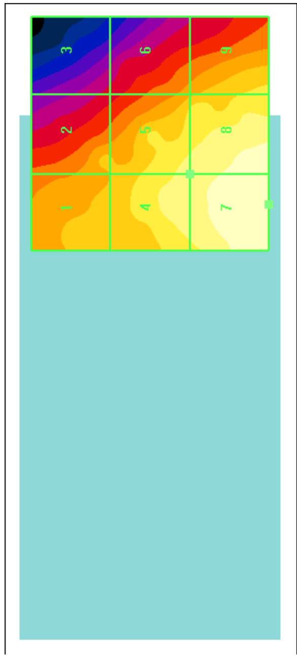
Figure 10-2 Sample H-field Scan Overlay
