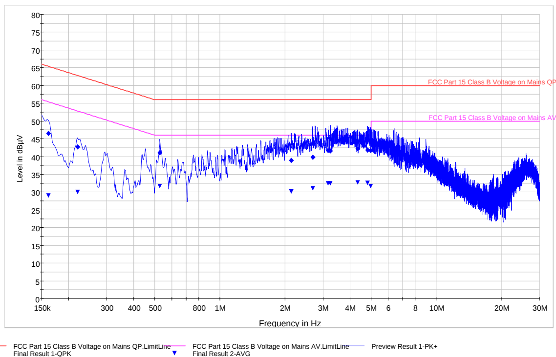
Plot 6-24. Line Conducted Plot with Bluetooth (L1)
