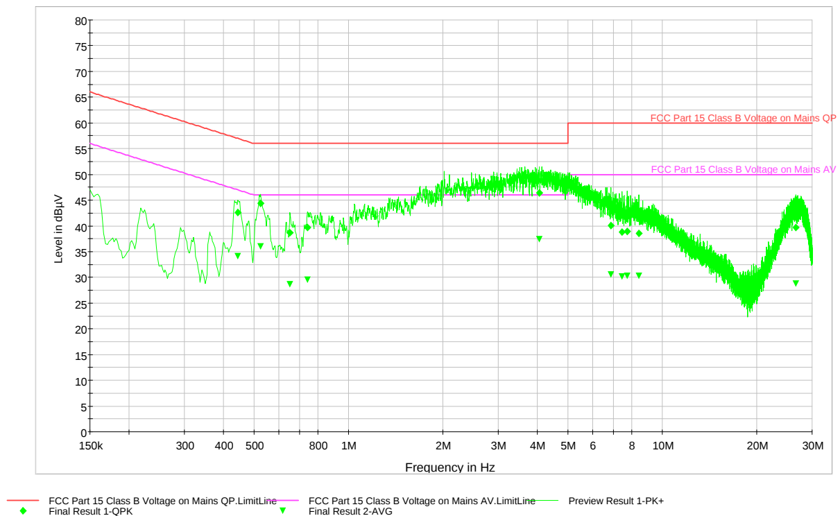
Plot 6-25. Line Conducted Data with Bluetooth (LN)
