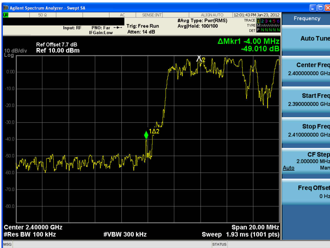
Plot 6-12. Band Edge Plot (Bluetooth with Hopping Enabled, 2Mbps – Ch. 0)
