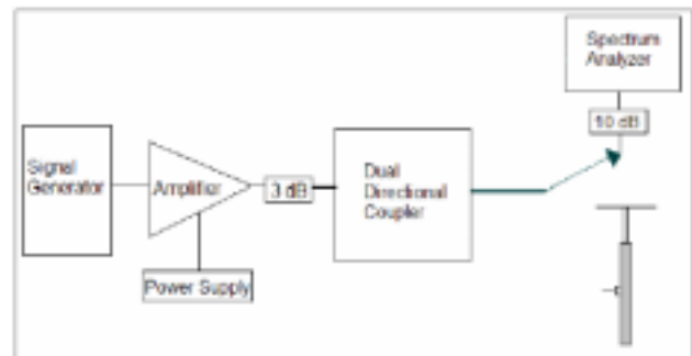
Figure 8.2 Setup to Peak Power using Spectrum Analyzer
