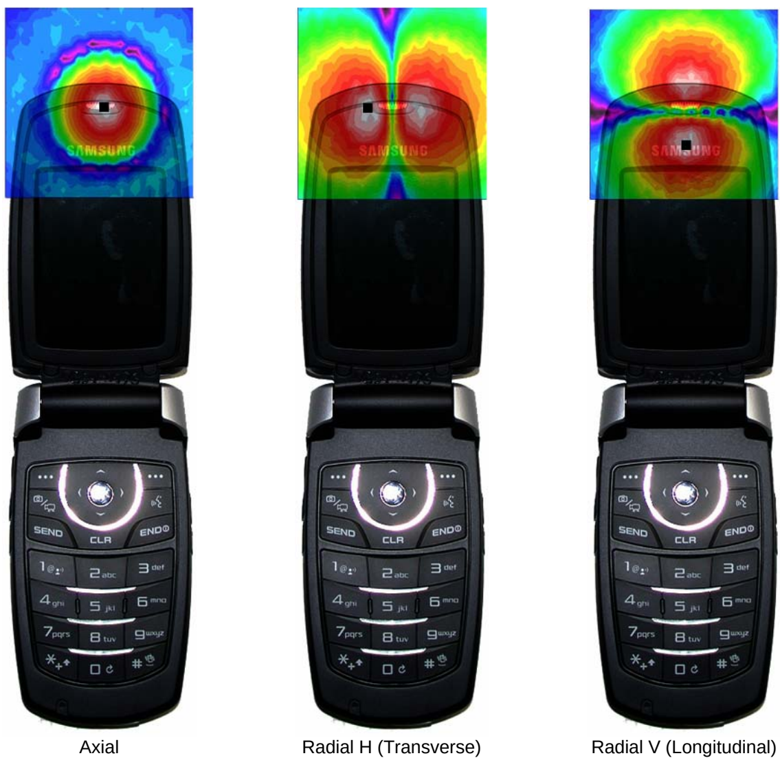
Figure 13-3 T-Coil Scan Overlay Magnetic Field Distributions
