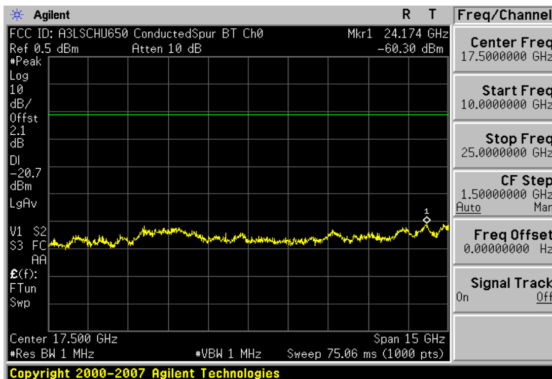
Plot 6-13. Conducted Spurious Plot (Bluetooth – Ch. 0)
