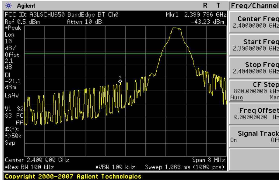
Plot 6-4. Band Edge Plot (Bluetooth – Ch. 0)
