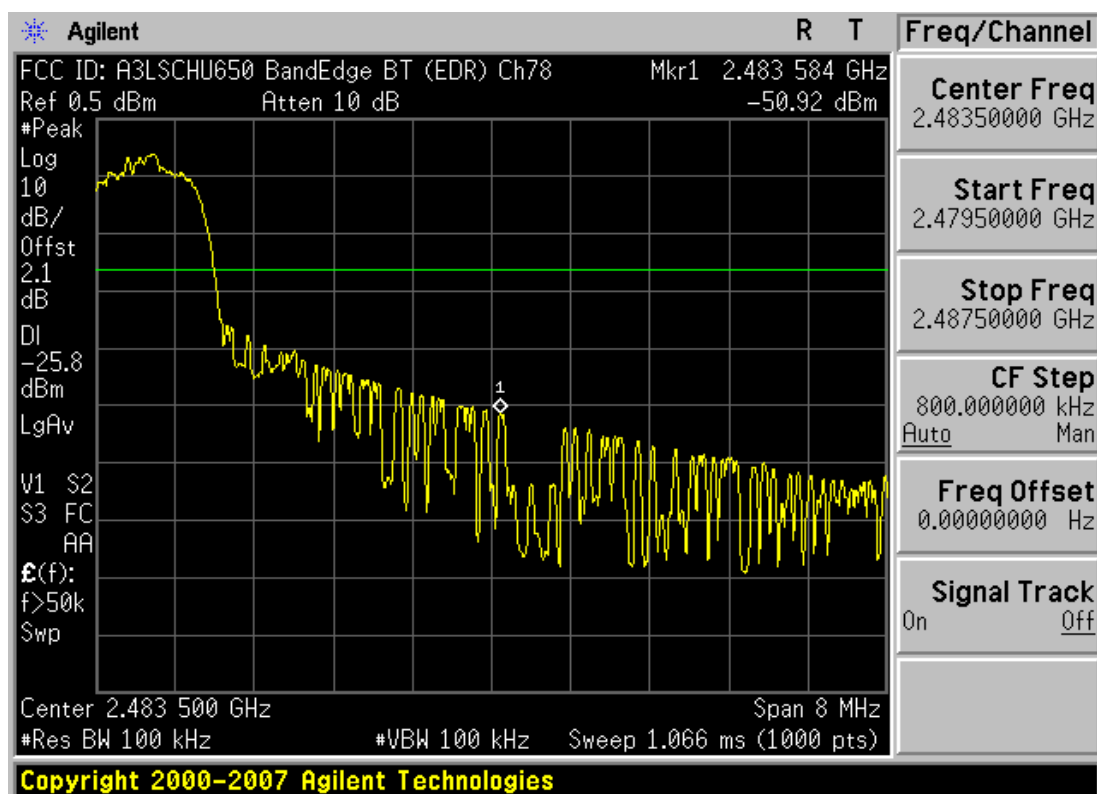
Plot 6-7. Band Edge Plot (Bluetooth 2.0 with Enhanced Data Rate – Ch. 78)
