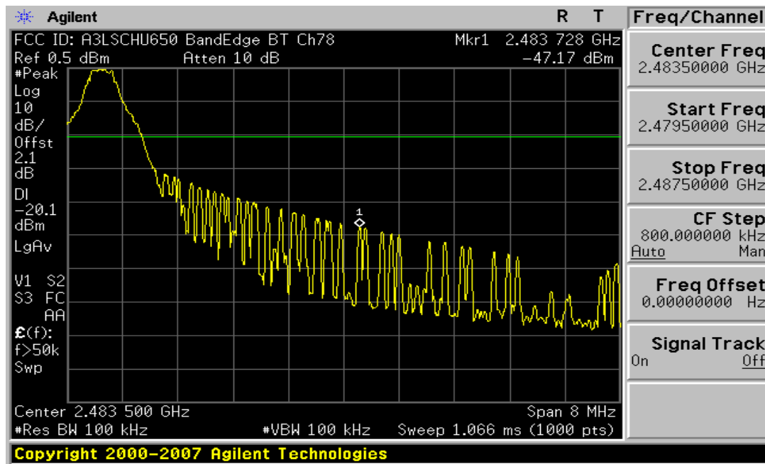
Plot 6-5. Band Edge Plot (Bluetooth – Ch. 78)
