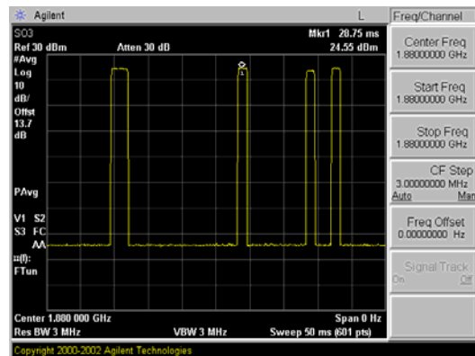
Figure 8-4 Zero-Span Plots
