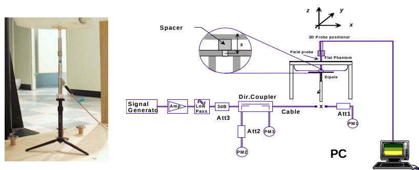
Figure 7.1 Dipole Validation Test Setup
