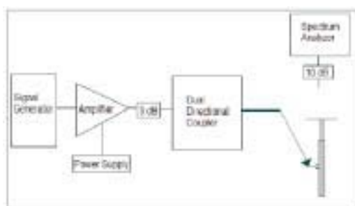
Figure 8.1 Setup to Dipole
