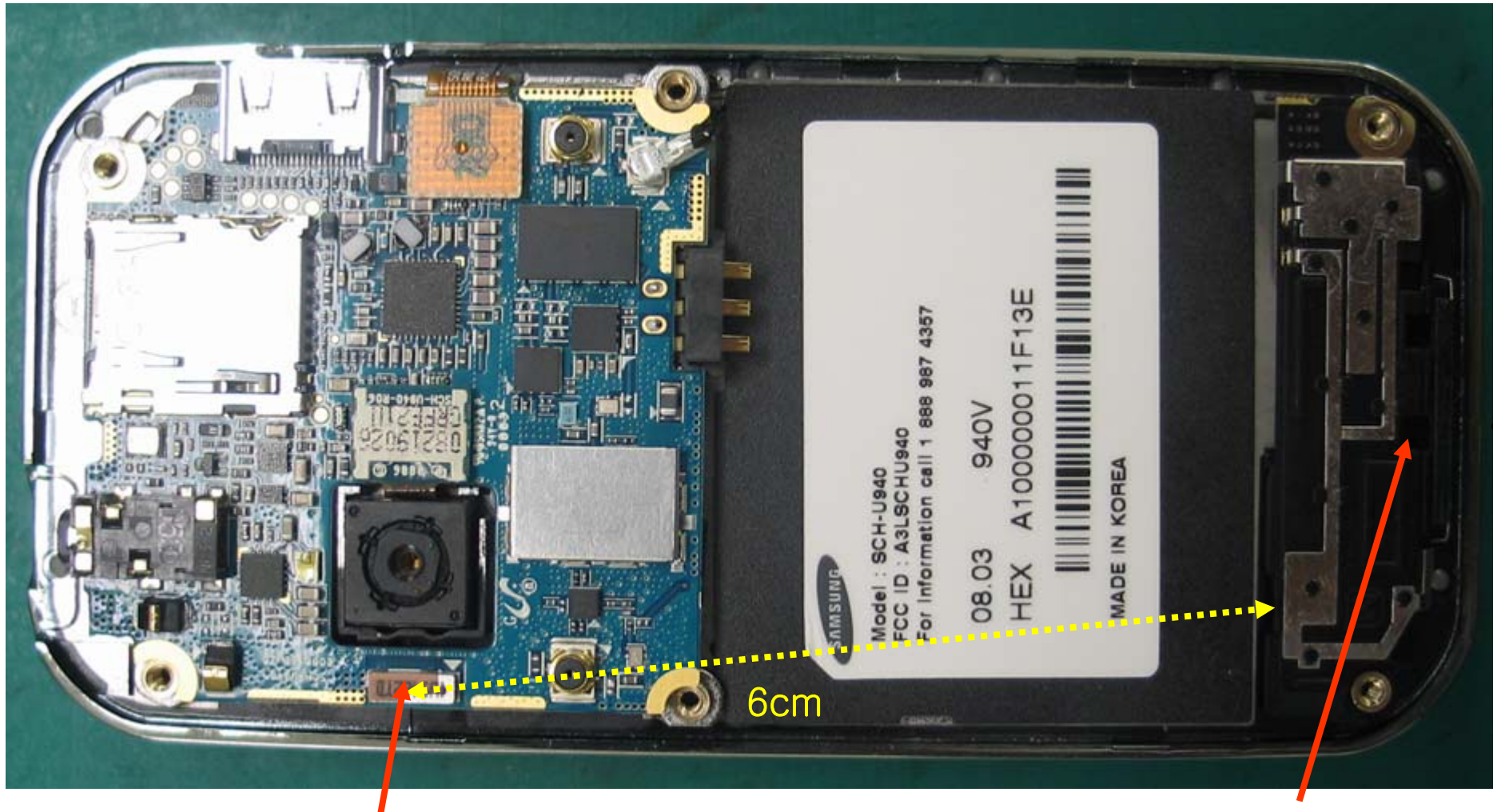
BT antenna
