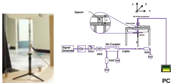
Figure 7.1 Dipole Validation Test Setup
