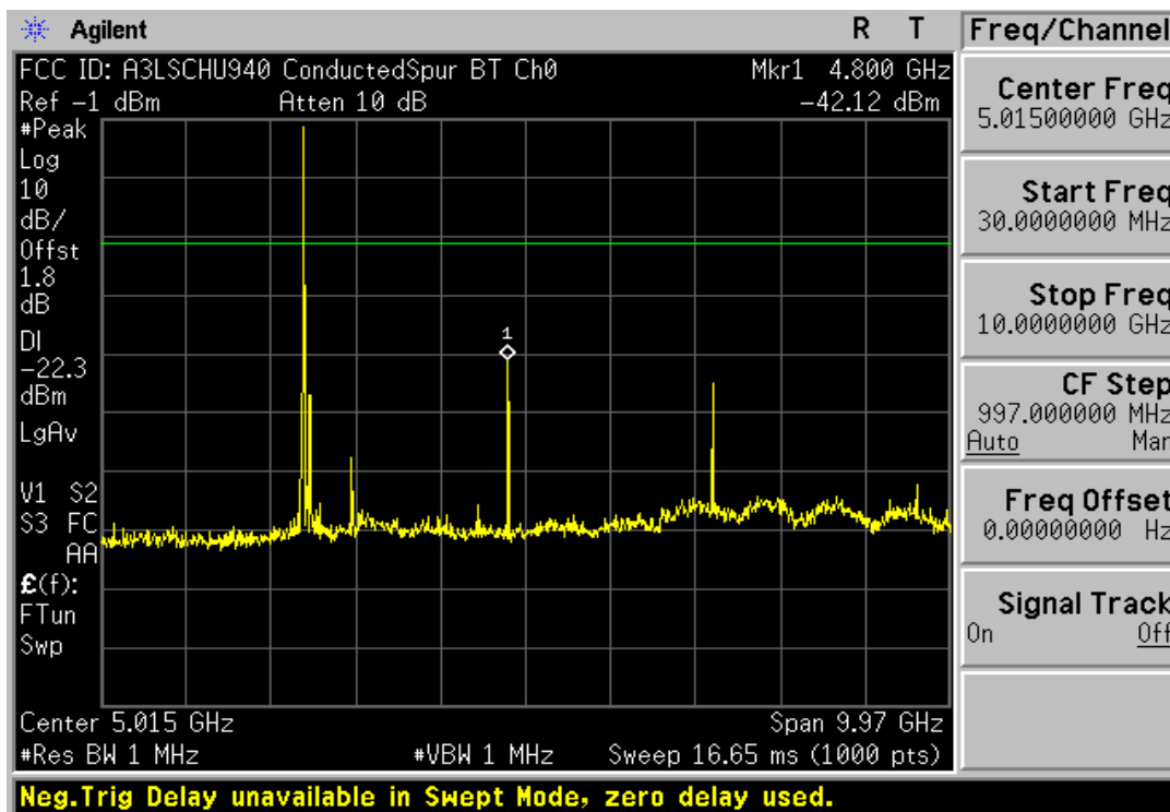
Plot 6-10. Conducted Spurious Plot (Bluetooth – Ch. 0)
