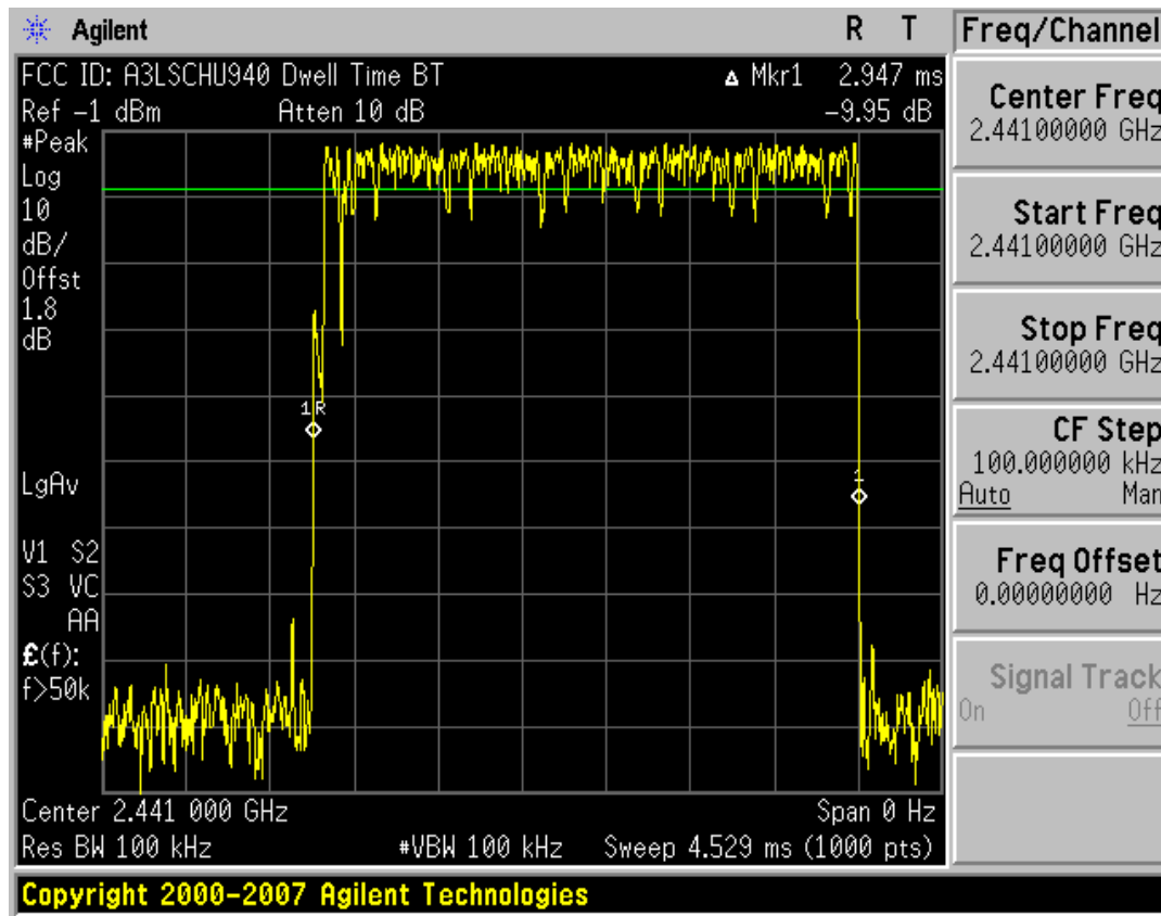
Plot 6-7. Time of Occupancy Plot (Bluetooth)
