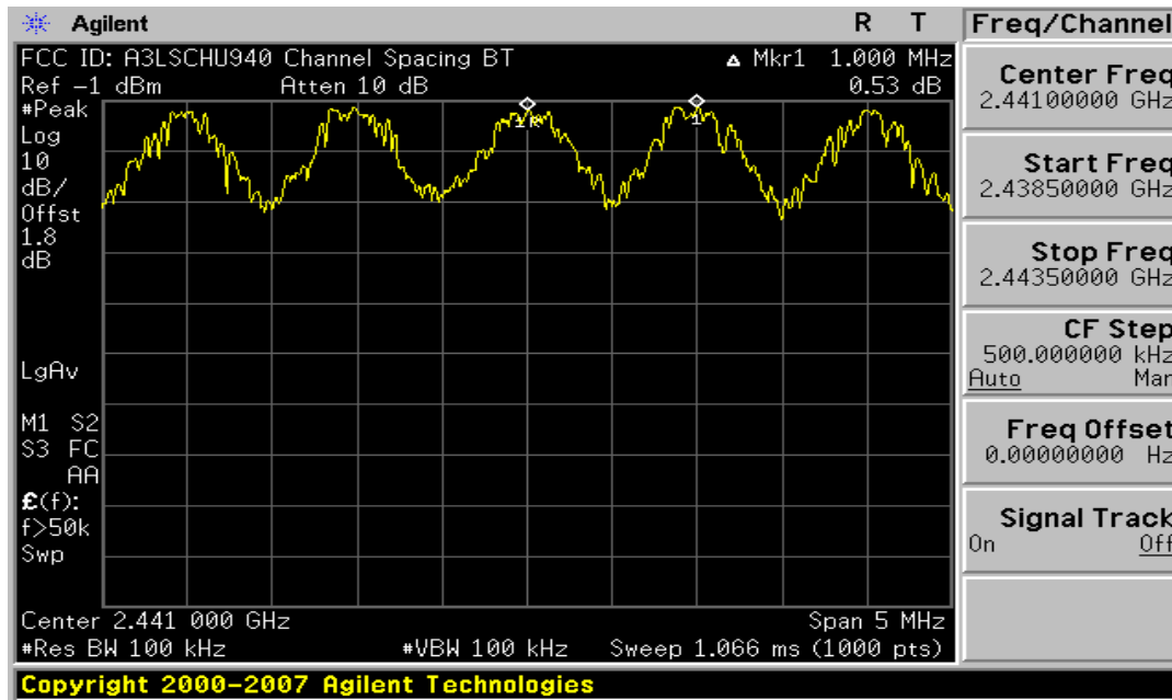
Plot 6-6. Channel Spacing Plot (Bluetooth)
