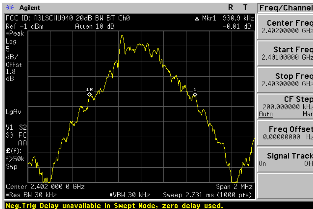
Plot 6-1. 20dB Bandwidth Plot (Bluetooth – Ch. 0)
