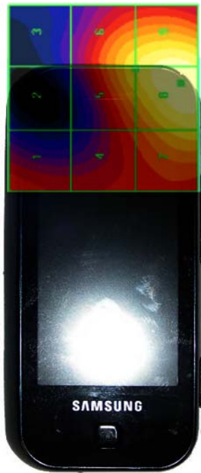
Figure 17-4 E-Field WD Scan overlay
