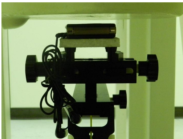
Front of the DUT with Phantom 1 cm Gap (with Headset)
