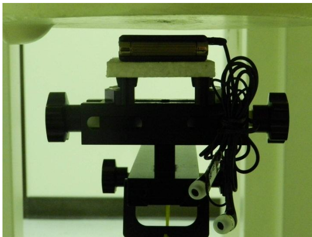
Back of the DUT with Phantom 1 cm Gap (with Headset)
