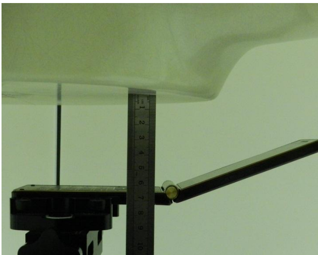
Jaw Region SAR - Flat Phantom_6.5cm
