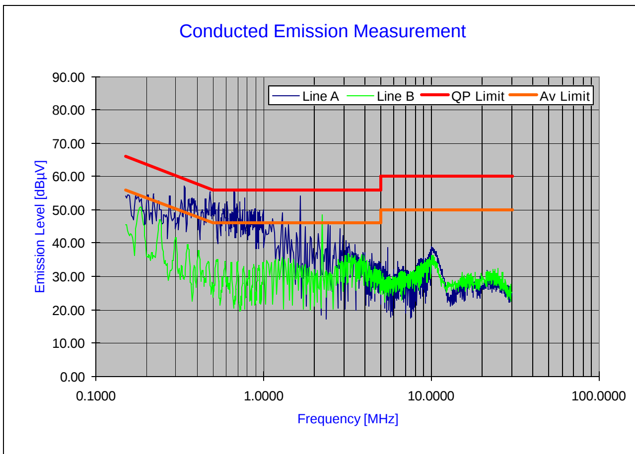
Plot 7-1. Line-Conducted Test Plot
