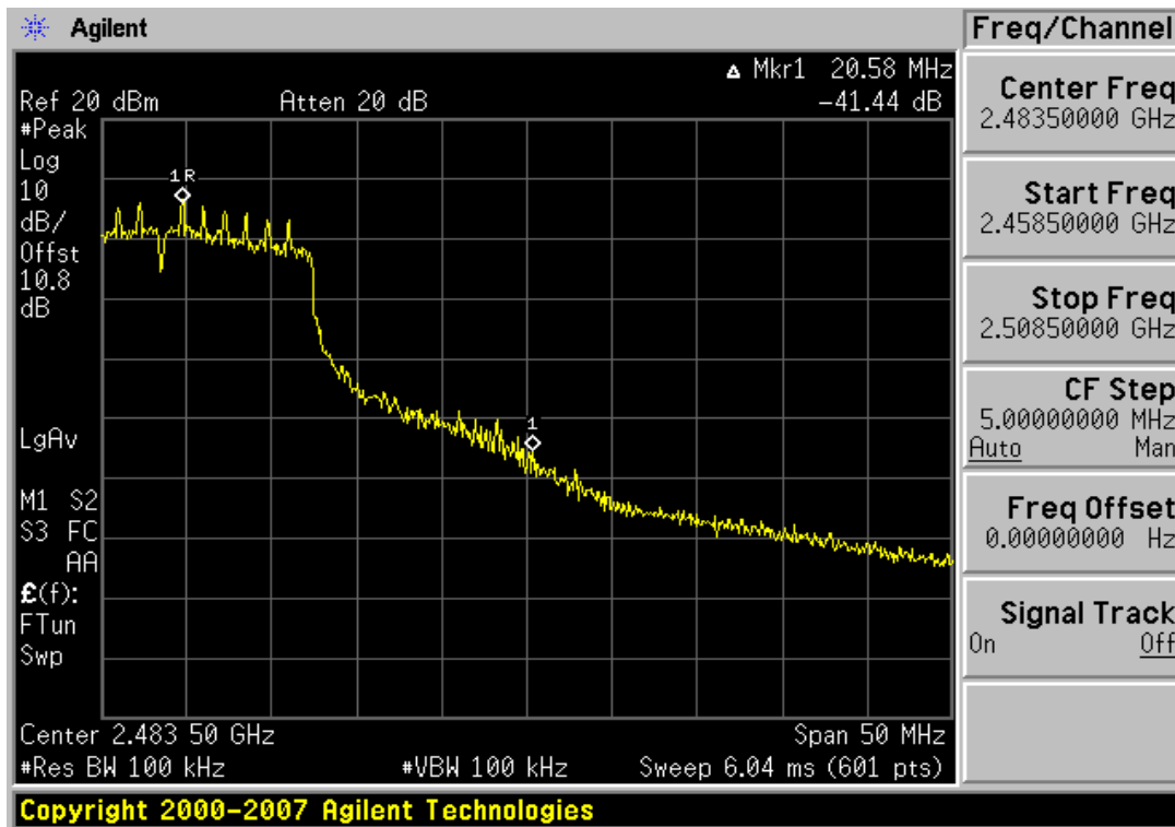
Plot 6-12. Band Edge Plot (802.11n – Ch. 11)
