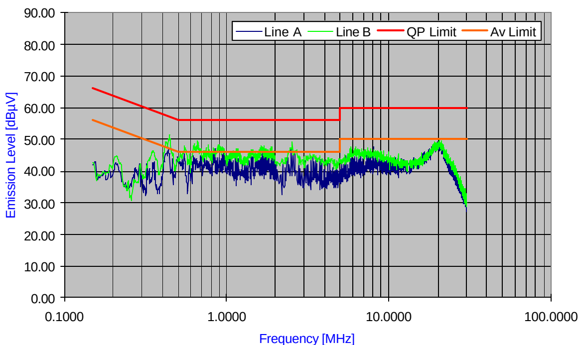
Plot 6-20. Line Conducted Plot with 802.11g
