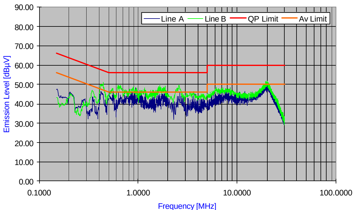
Plot 6-19. Line Conducted Plot with 802.11b
