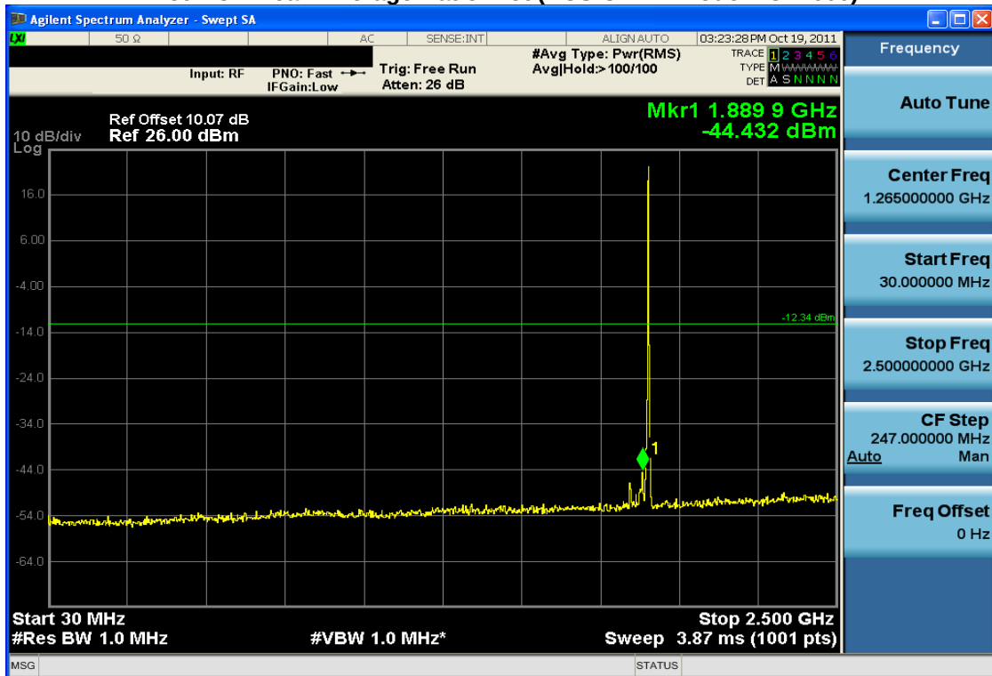
Plot 7-32. Conducted Spurious Plot (PCS CDMA Mode – Ch. 1175)
