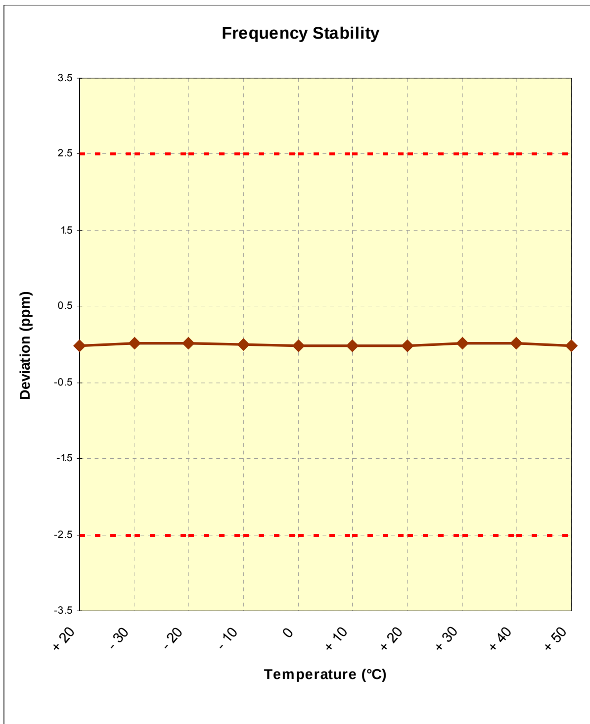
Figure 6-2. Frequency Stability Graph (PCS GSM Mode – Ch. 661)
