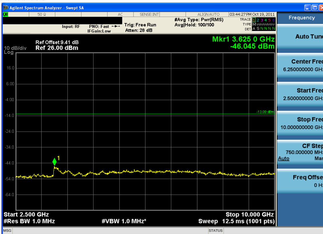
Plot 7-21. Conducted Spurious Plot (Cellular CDMA Mode – Ch. 777)
