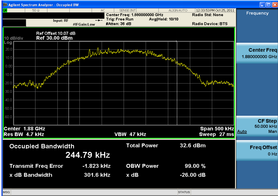
Plot 7-11. Occupied Bandwidth Plot (EDGE1900 Mode – Ch. 661)
