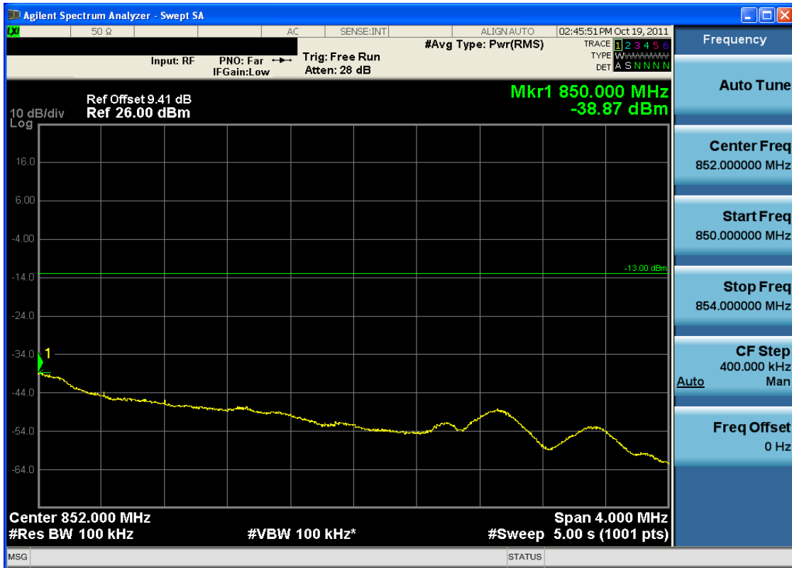
Plot 7-23. 4MHz Span Plot (Cellular CDMA Mode – Ch. 777)
