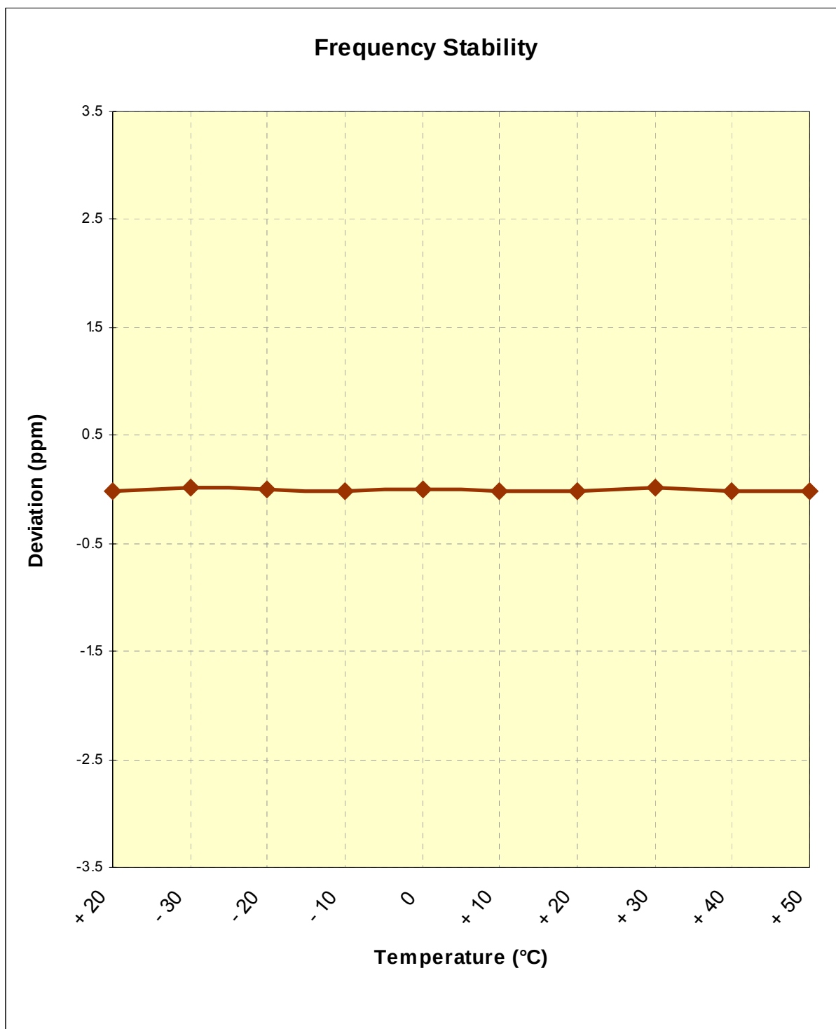
Figure 6-3. Frequency Stability Graph (PCS CDMA Mode – Ch. 600)
