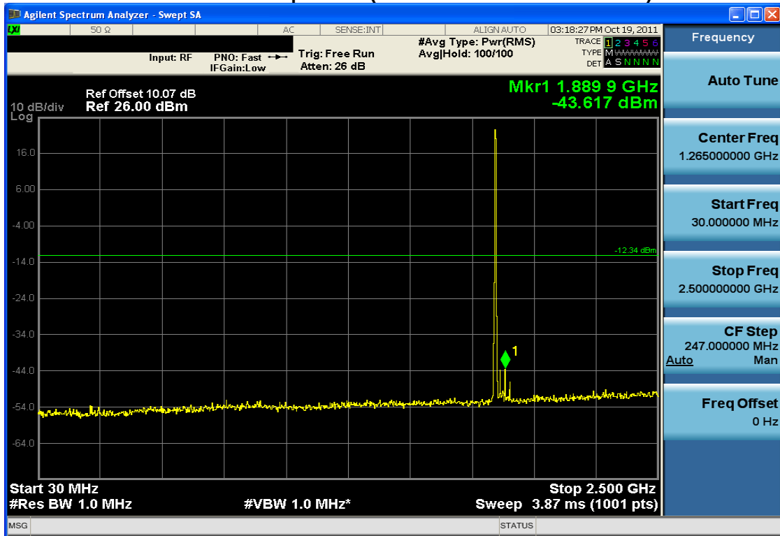
Plot 7-24. Conducted Spurious Plot (PCS CDMA Mode – Ch. 25)
