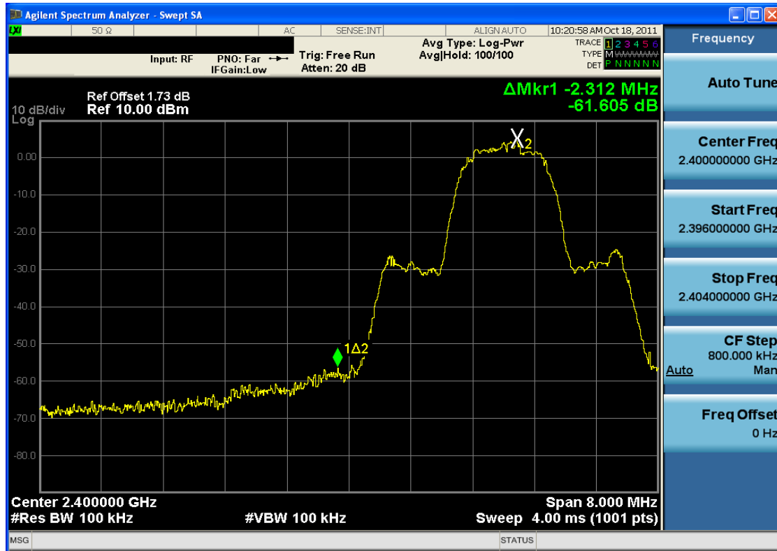
Plot 6-10. Band Edge Plot (Bluetooth, 3Mbps – Ch. 0)
