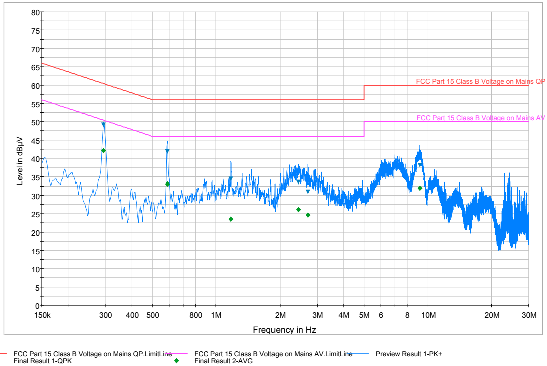
Plot 6-7. Line-Conducted Test Plot (N)
