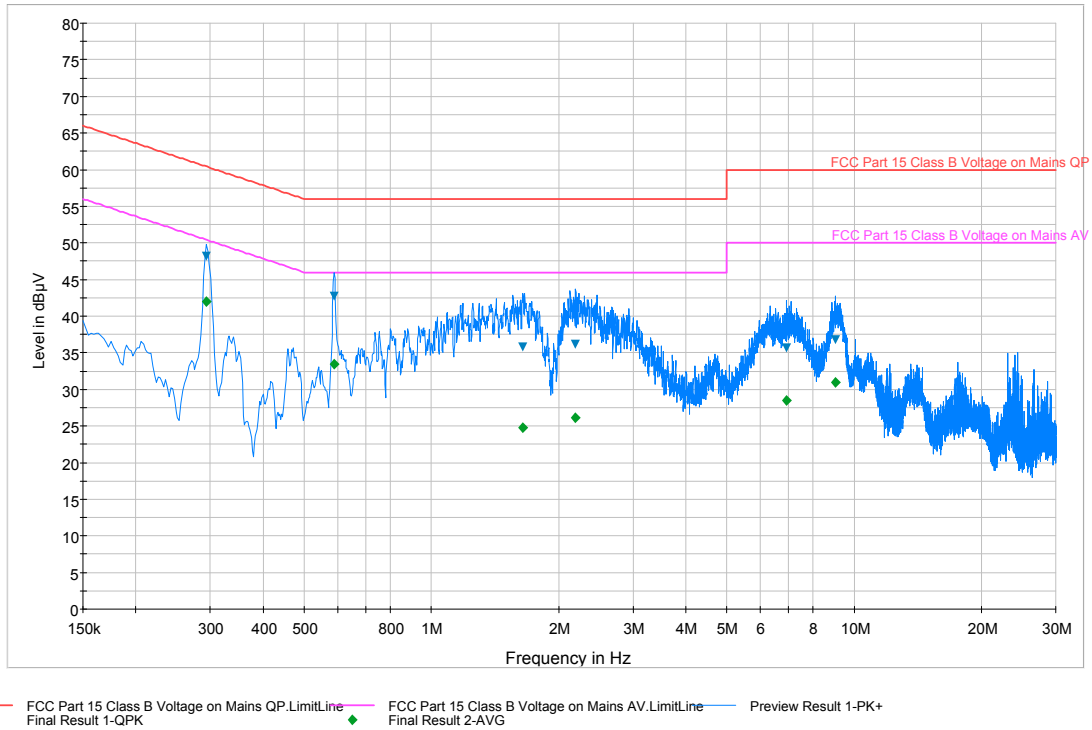
Plot 6-6. Line-Conducted Test Plot (L1)
