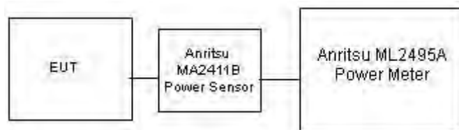
Figure 9-3 Power Measurement Setup for SISO Bandwidths < 50 MHz
