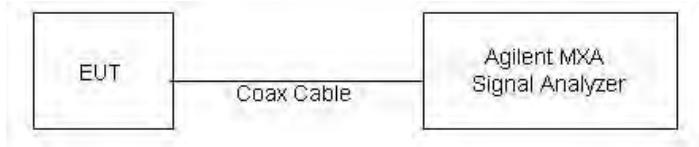
Figure 9-4 Power Measurement Setup for SISO Bandwidths > 50 MHz
