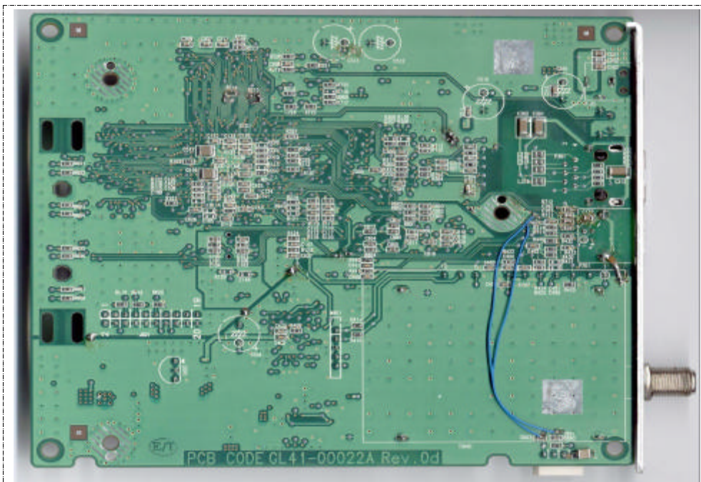
Solder view of main b'd
