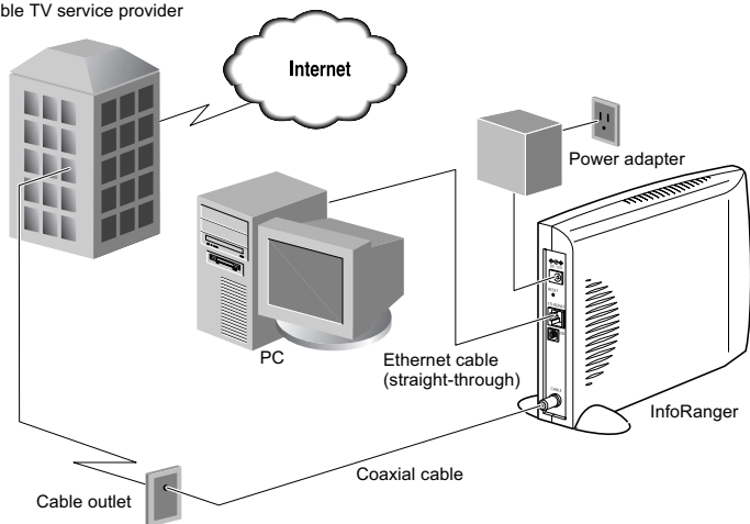
Figure 3-9 Cable connection in case of a singal PC connection
