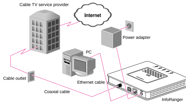
Figure 1-2 Network connection if you only subscribe to a cable Internet service
