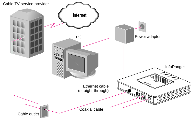
Figure 3-9 Cable connection in case of a single PC connection
