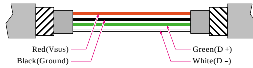
Figure D-7 USB Connector Termination
