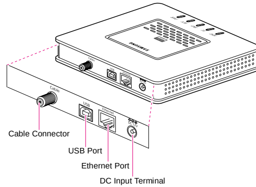
Figure 4-2 Rear View of the InfoRanger
