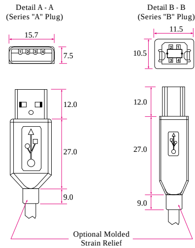
Figure D-9 Pin Signals of the USB cable
