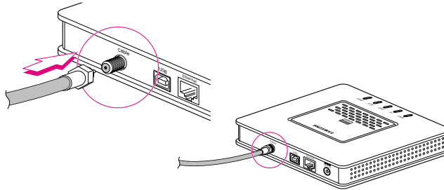
Figure 3-4 Connecting the coaxial cable to the Cable connector
