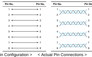
Figure D-3 Pin Signals of the straight-through cable
