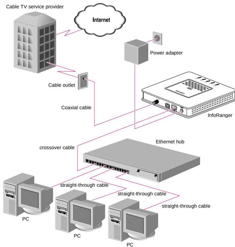
Figure 3-10 Cable connection in case of multiple PCs connection
