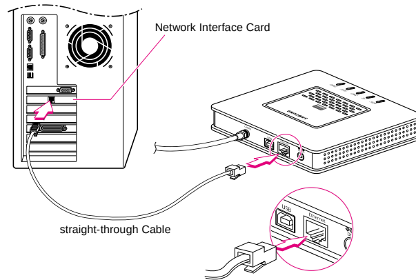
Figure 3-5 Connecting the RJ-45 Ethernet cable to the Ethernet port and a PC
