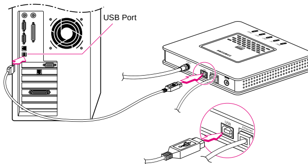
Figure 3-6 Connecting the USB cable to the USB port and a PC
