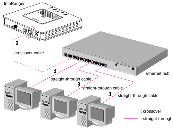
Figure 3-7 Connecting the InfoRanger to multiple PCs through an Ethernet hub
