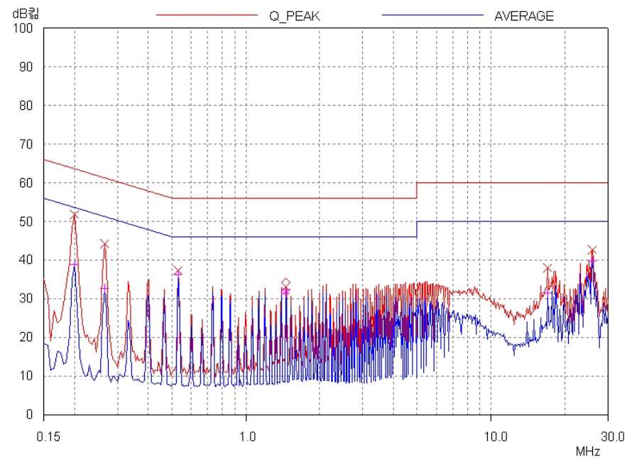
NEUTRAL LINE
