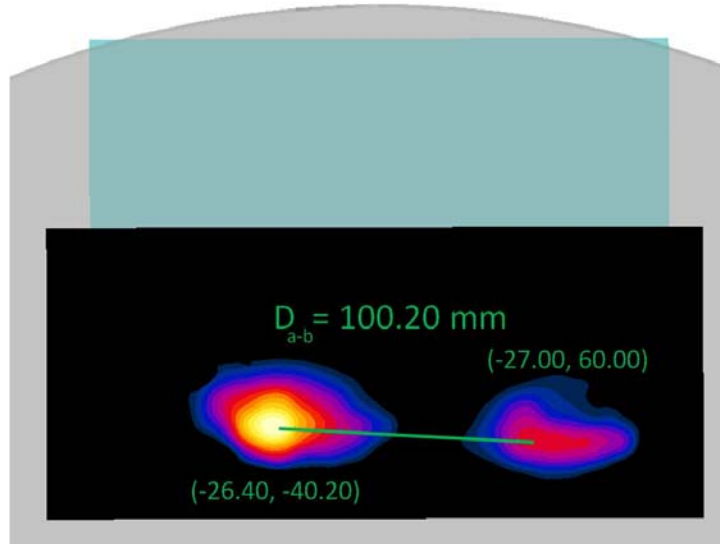
Figure 11-4 Peak SAR Locations for Body Back Side at 0.0 cm LTE Band 17 and 2.4 GHz WLAN Antenna 2
