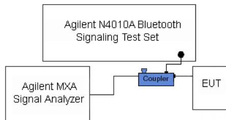
Figure 8-5 Power Measurement Setup
