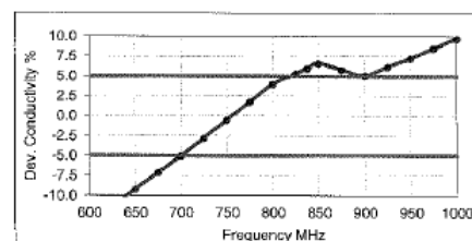
Figure 16-2 750MHz Body Tissue Equivalent Matter
