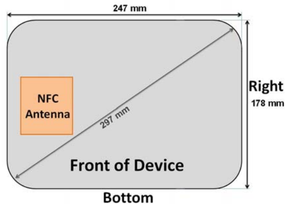
Figure 1-2 NFC Antenna Locations
