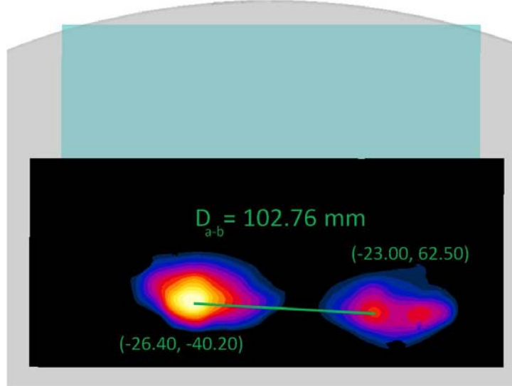
Figure 11-3 Peak SAR Locations for Body Back Side at 0.0 cm GPRS 1900 and 2.4 GHz WLAN Antenna 2
