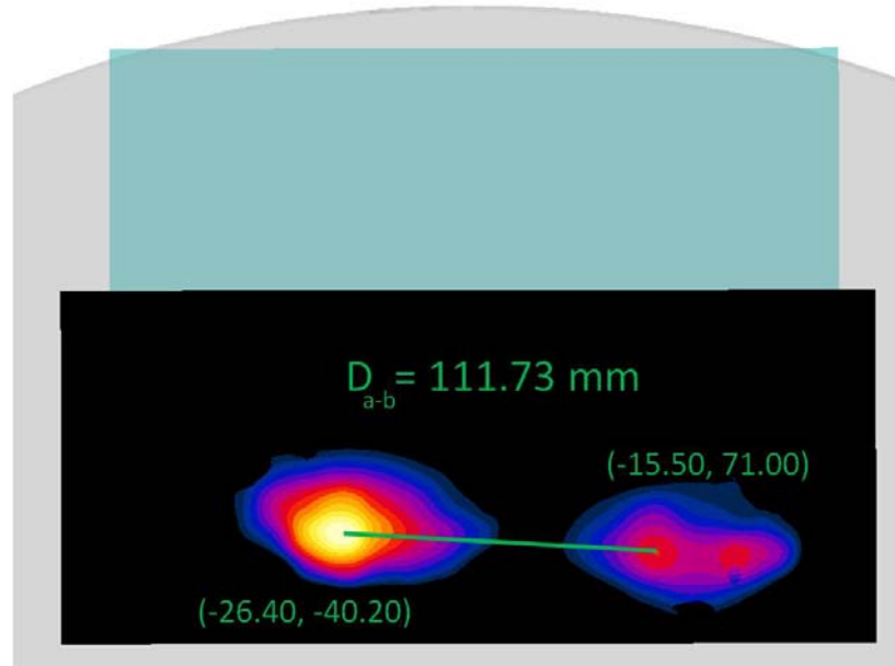
Figure 11-2 Peak SAR Locations for Body Back Side at 0.0 cm GPRS 850 and 2.4 GHz WLAN Antenna 2
