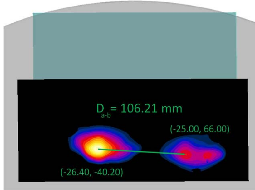
Figure 11-1 Peak SAR Locations for Body Back Side at 0.0 cm UMTS 850 and 2.4 GHz WLAN Antenna 2
