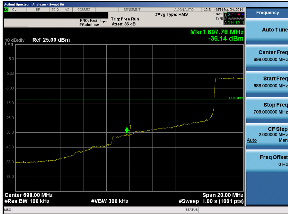
Plot 6-13. Lower Band Edge Plot (Band 17 – 10.0MHz QPSK – RB Size 50)
