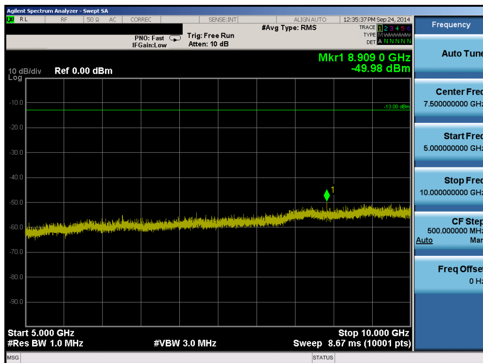
Plot 6-10. Conducted Spurious Plot (Band 17 – 10.0MHz QPSK – RB Size 1, RB Offset 0 – High Channel)
