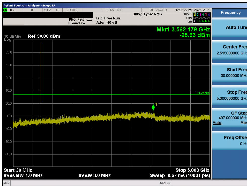
Plot 6-9. Conducted Spurious Plot (Band 17 – 10.0MHz QPSK – RB Size 1, RB Offset 0 – High Channel)
