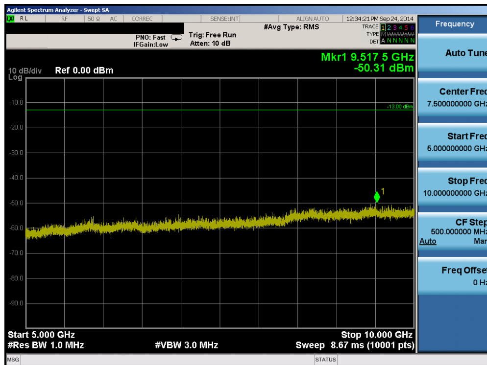
Plot 6-6. Conducted Spurious Plot (Band 17 – 10.0MHz QPSK – RB Size 1, RB Offset 0 – Low Channel)
