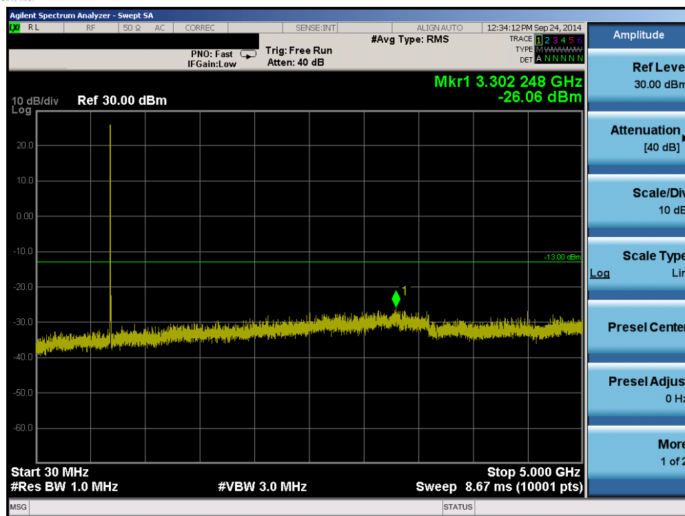
Plot 6-5. Conducted Spurious Plot (Band 17 – 10.0MHz QPSK – RB Size 1, RB Offset 0– Low Channel)
