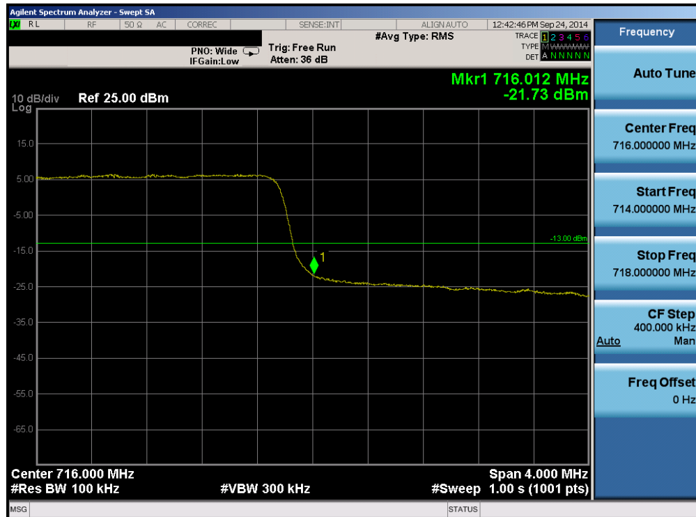
Plot 6-12. Upper Band Edge Plot (Band 17 – 5.0MHz QPSK – RB Size 25)
