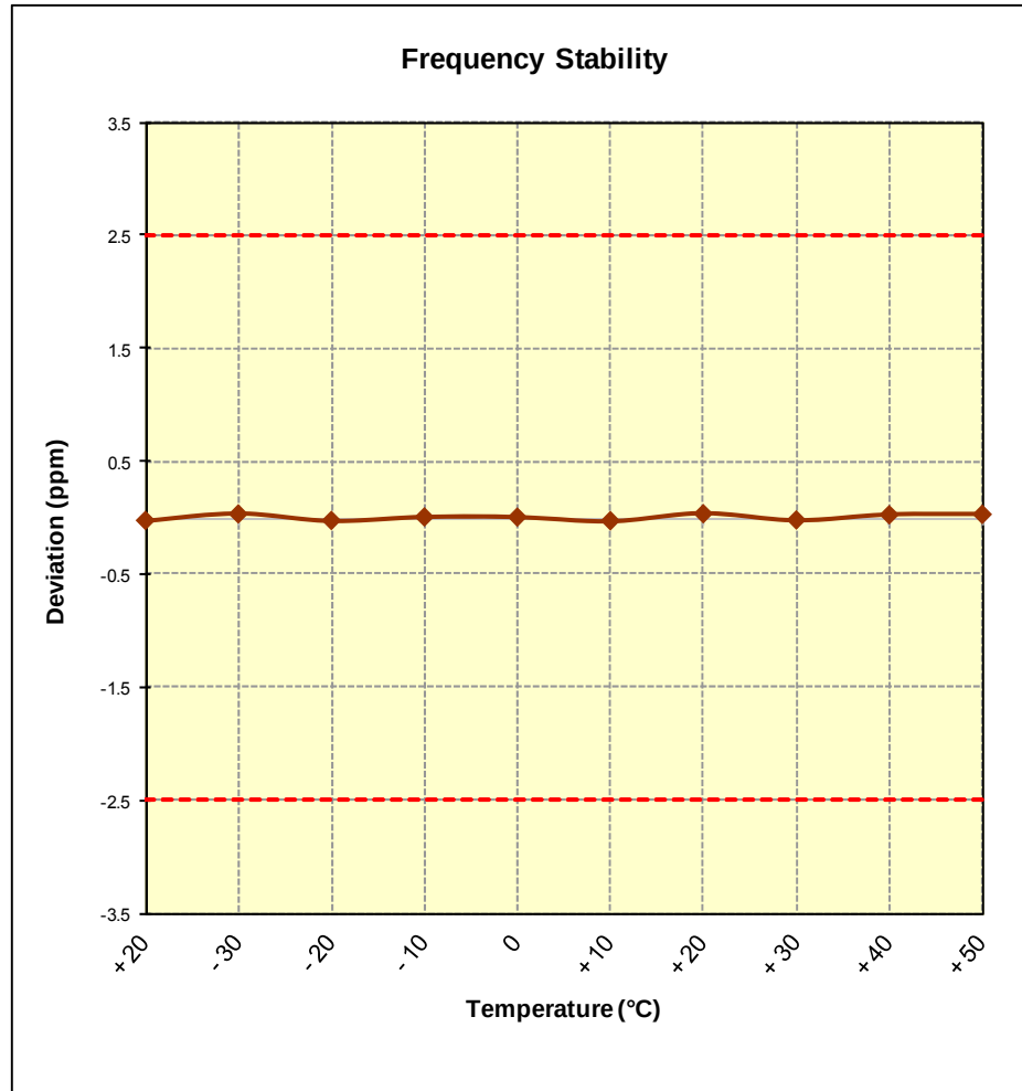
Figure 6-8. Frequency Stability Graph (Cellular WCDMA Mode – Ch. 4183)
