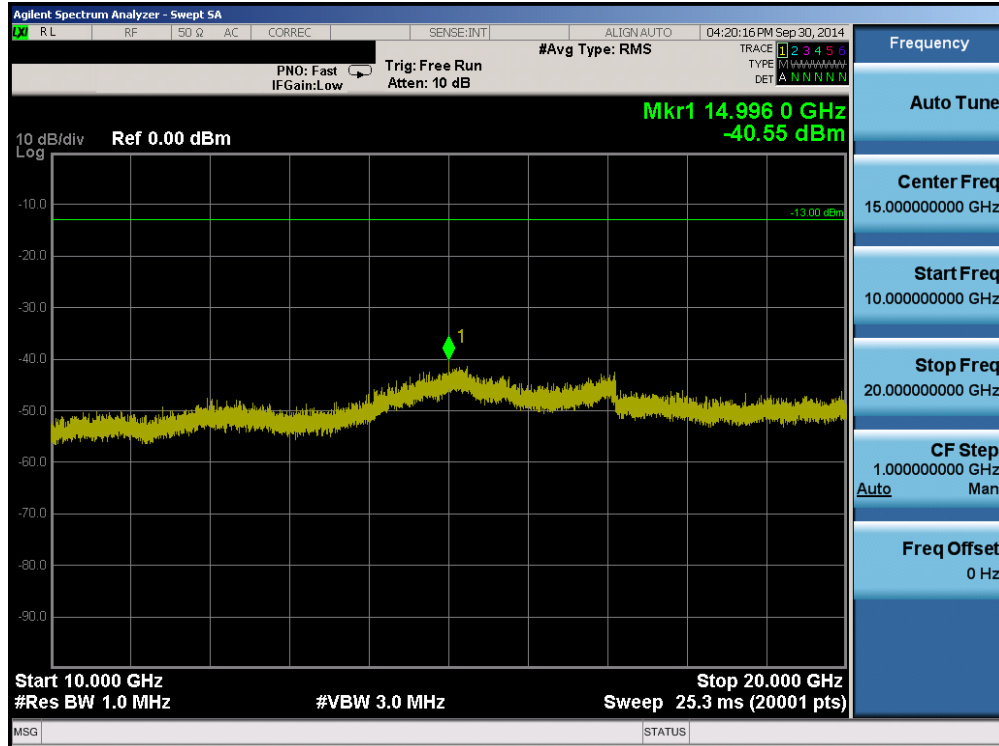
Plot 6-20. Conducted Spurious Plot (PCS GPRS Mode – Ch. 810)
