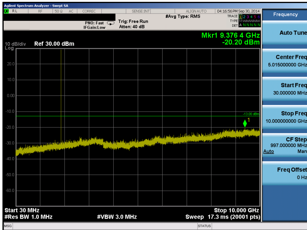
Plot 6-17. Conducted Spurious Plot (PCS GPRS Mode – Ch. 661)
