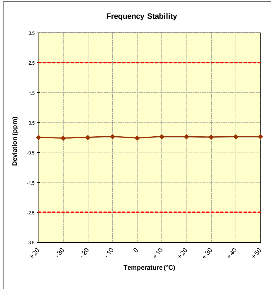
Figure 6-7. Frequency Stability Graph (Cellular GPRS Mode – Ch. 190)
