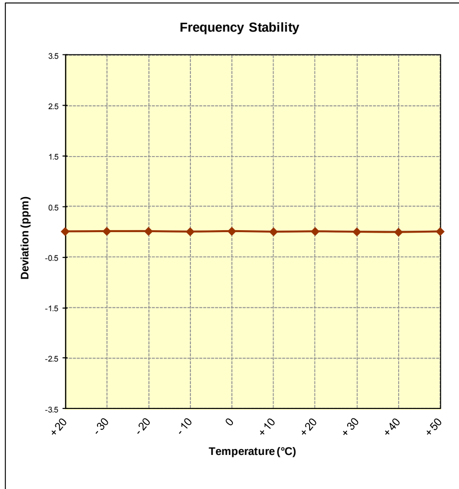
Figure 6-9. Frequency Stability Graph (PCS GPRS Mode – Ch. 661)
