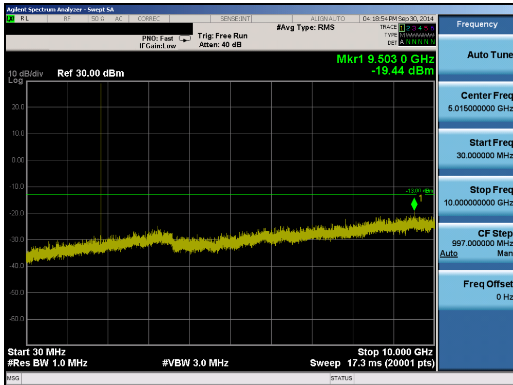
Plot 6-15. Conducted Spurious Plot (PCS GPRS Mode – Ch. 512)
