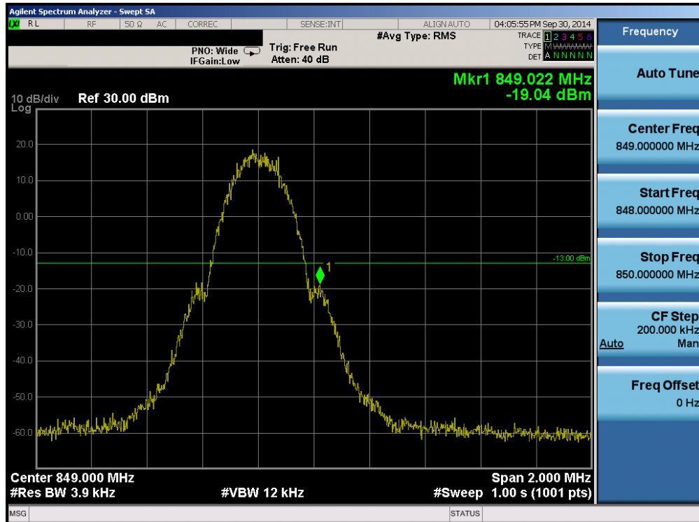
Plot 6-28. Band Edge Plot (Cellular GPRS Mode – Ch. 251)
