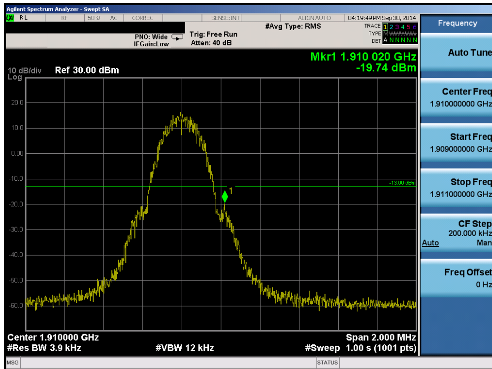
Plot 6-30. Band Edge Plot (PCS GPRS Mode – Ch. 810)
