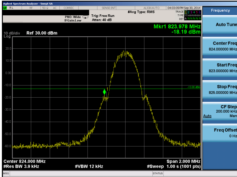
Plot 6-27. Band Edge Plot (Cellular GPRS Mode – Ch. 128)
