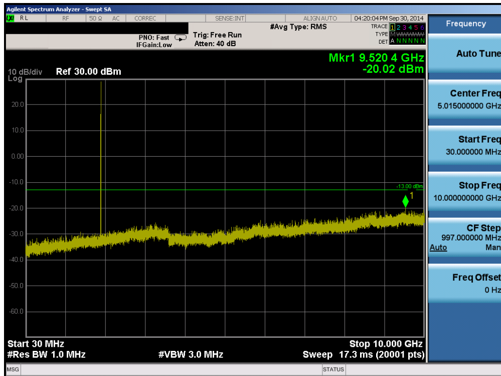
Plot 6-19. Conducted Spurious Plot (PCS GPRS Mode – Ch. 810)
