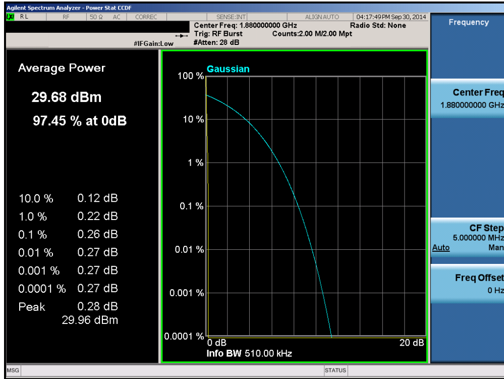
Plot 6-33. Peak-Average Ratio Plot (PCS GPRS Mode – Ch. 661)
