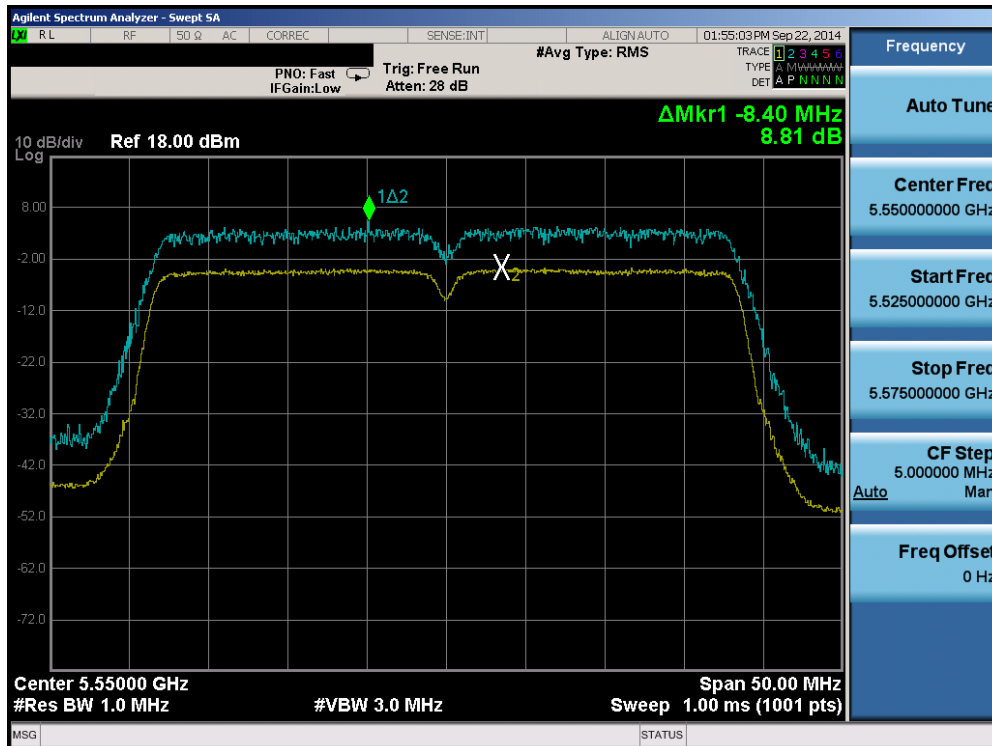
Plot 6-127. Peak Excursion Ratio Plot (40MHz BW 802.11n (UNII Band 2C) – Ch. 110)
