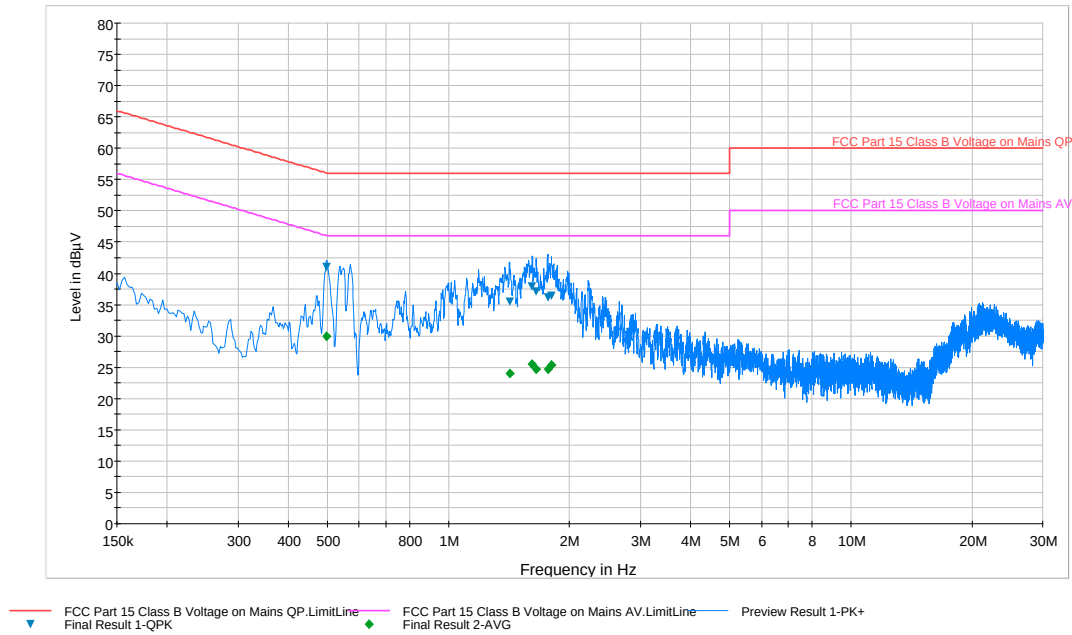
Plot 6-192. Line Conducted Plot with 802.11a UNII Band 2A (N)
