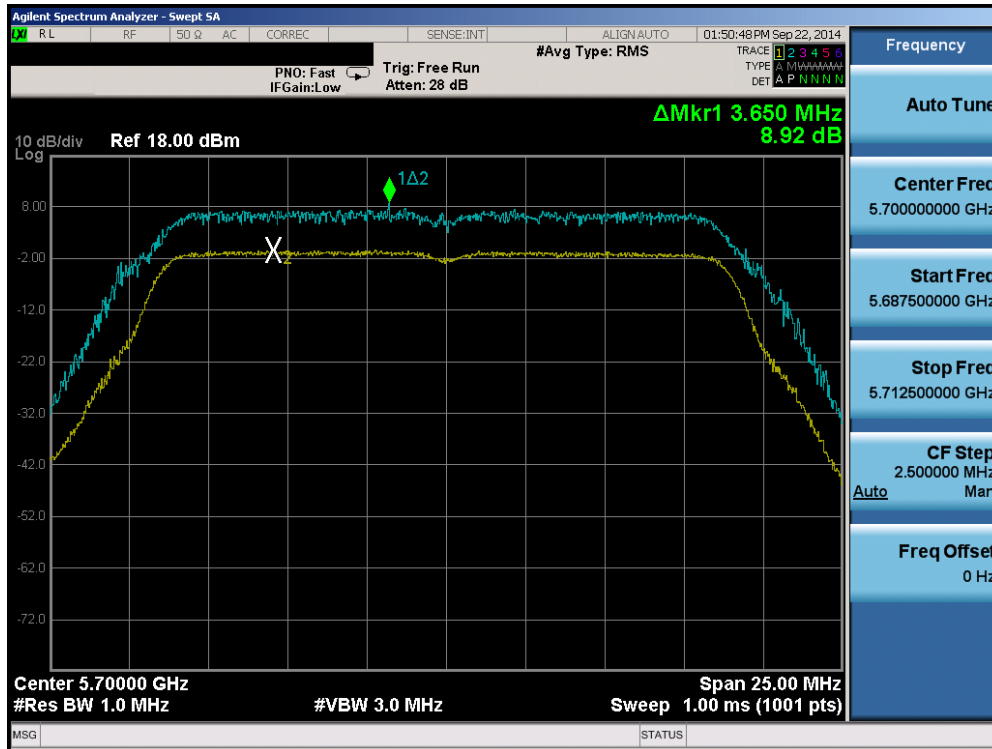
Plot 6-126. Peak Excursion Ratio Plot (20MHz BW 802.11n (UNII Band 2C) – Ch. 140)
