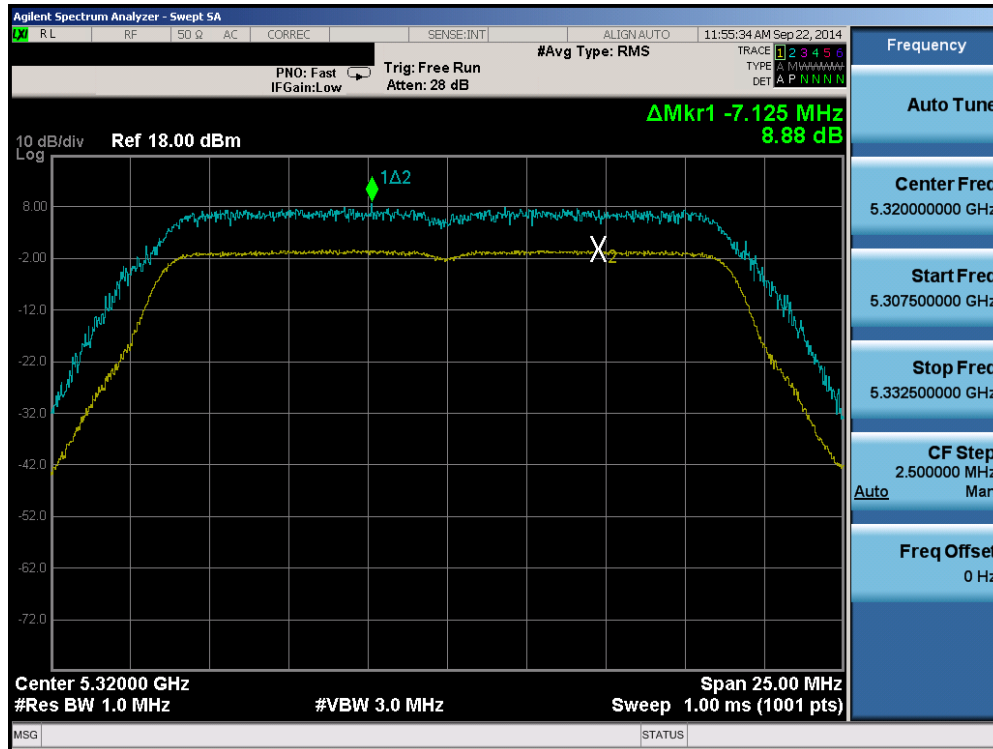
Plot 6-122. Peak Excursion Ratio Plot (20MHz BW 802.11n (UNII Band 2A) – Ch. 64)
