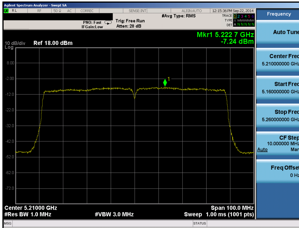
Plot 6-73. Peak Power Spectral Density Plot (80MHz BW 802.11ac (UNII Band 1) – Ch. 42)
