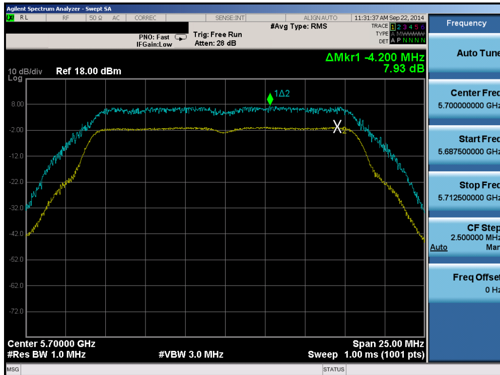
Plot 6-123. Peak Excursion Ratio Plot (802.11a (UNII Band 2C) – Ch. 140)
