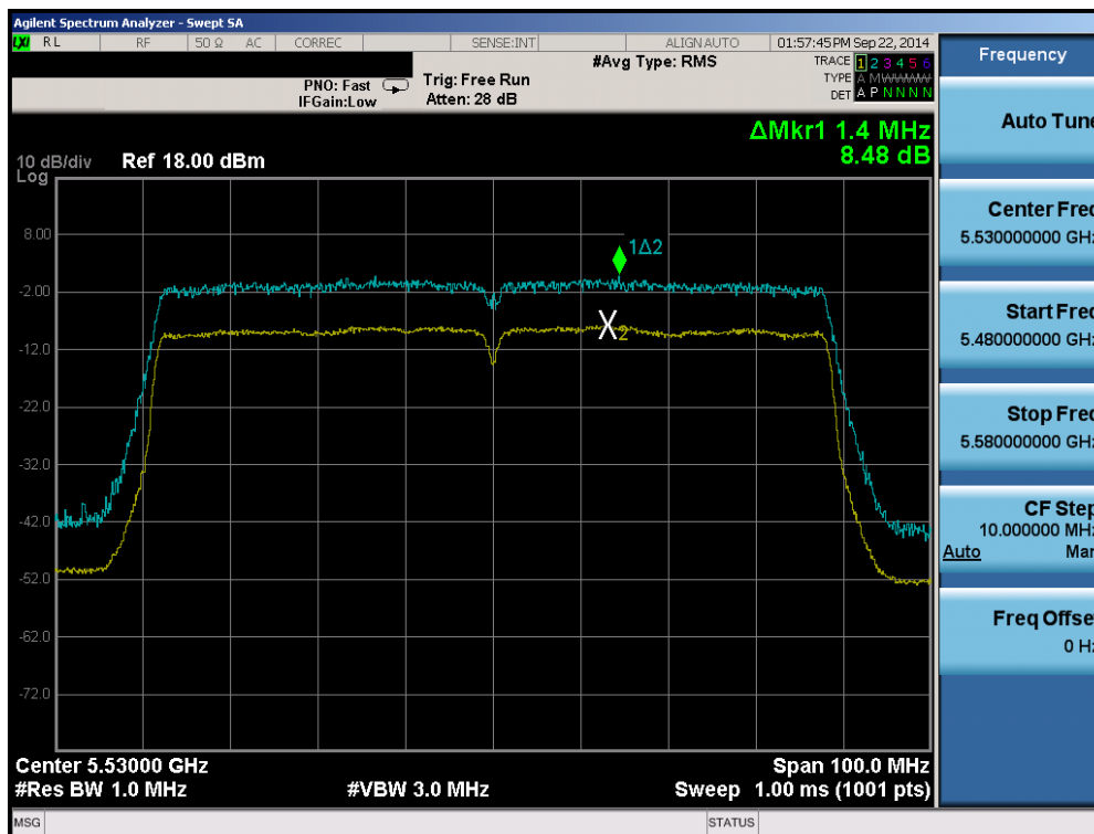
Plot 6-128. Peak Excursion Ratio Plot (80MHz BW 802.11ac (UNII Band 2C) - Ch. 106)
