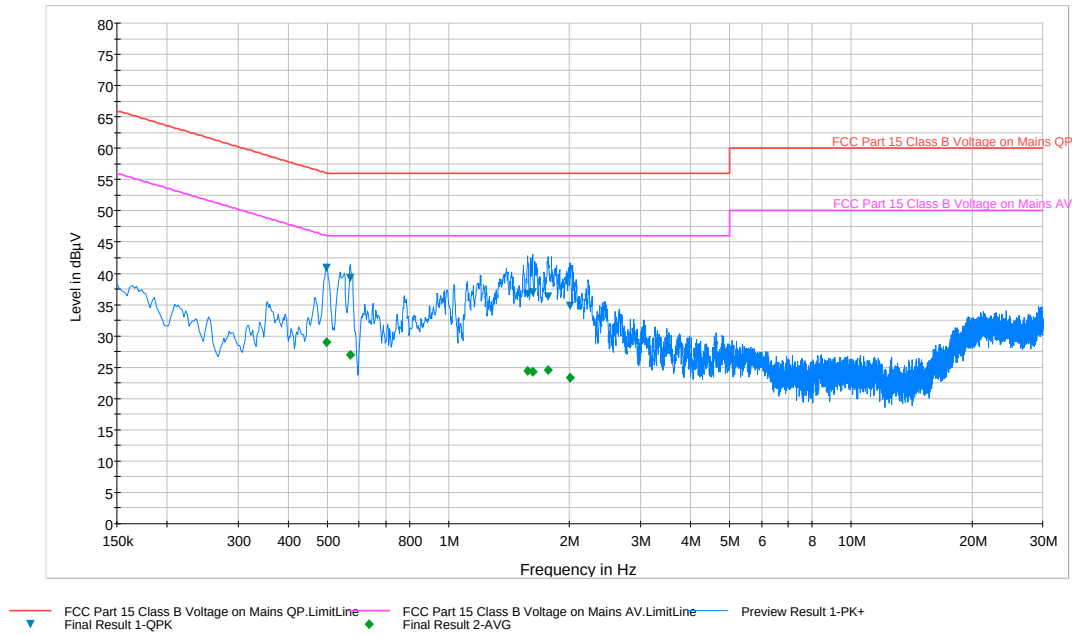
Plot 6-194. Line Conducted Plot with 802.11a UNII Band 2C (N)
