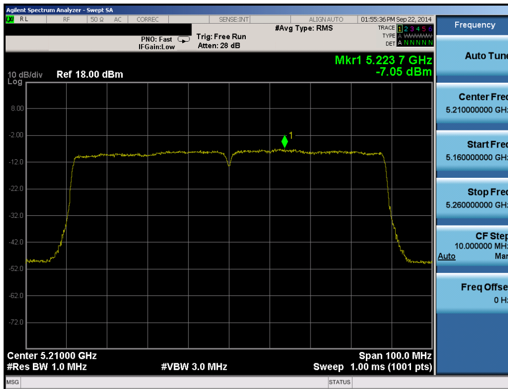
Plot 6-101. Peak Power Spectral Density Plot (80MHz BW 802.11ac (UNII Band 1) – Ch. 42)
