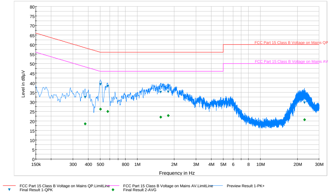
Plot 6-193. Line Conducted Plot with 802.11a UNII Band 2C (L1)
