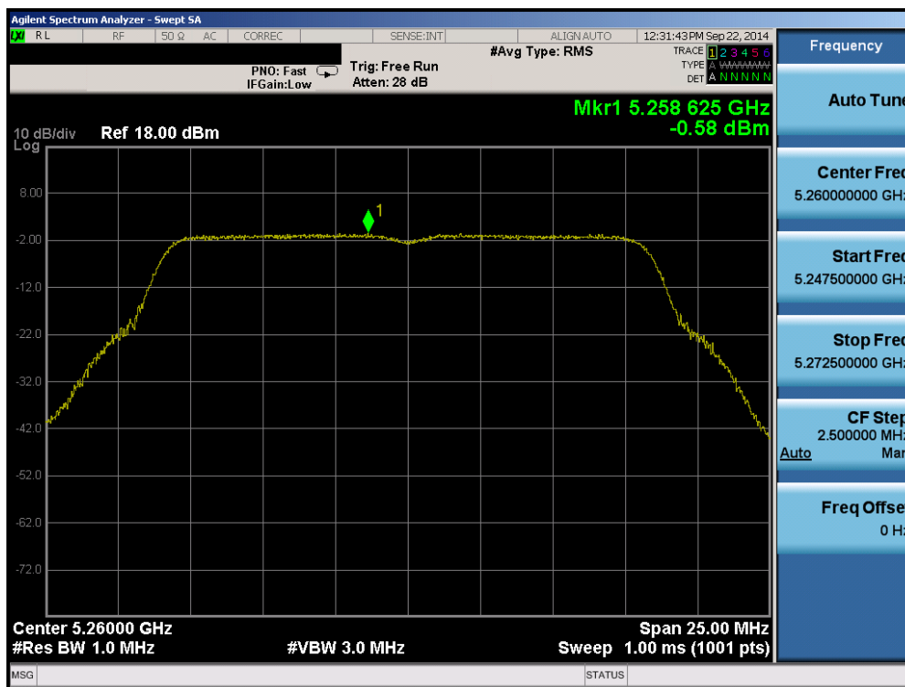
Plot 6-102. Peak Power Spectral Density Plot (802.11a (UNII Band 2A) – Ch. 52)
