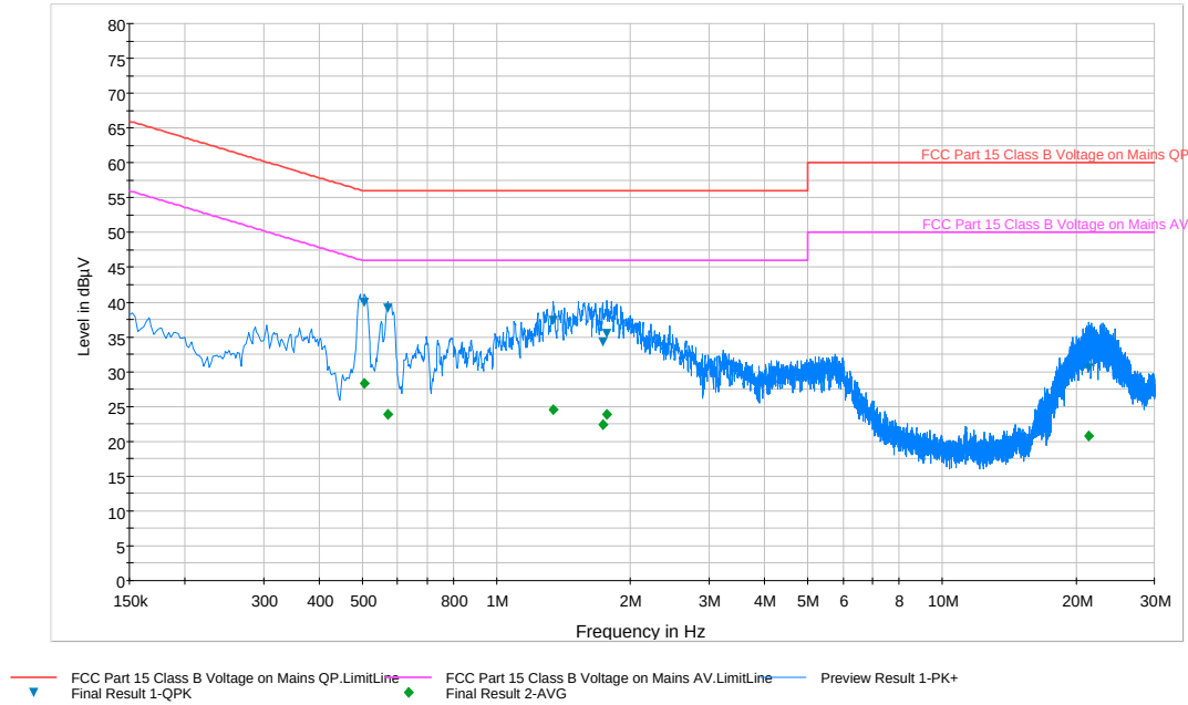
Plot 6-189. Line Conducted Plot with 802.11a UNII Band 1 (L1)
