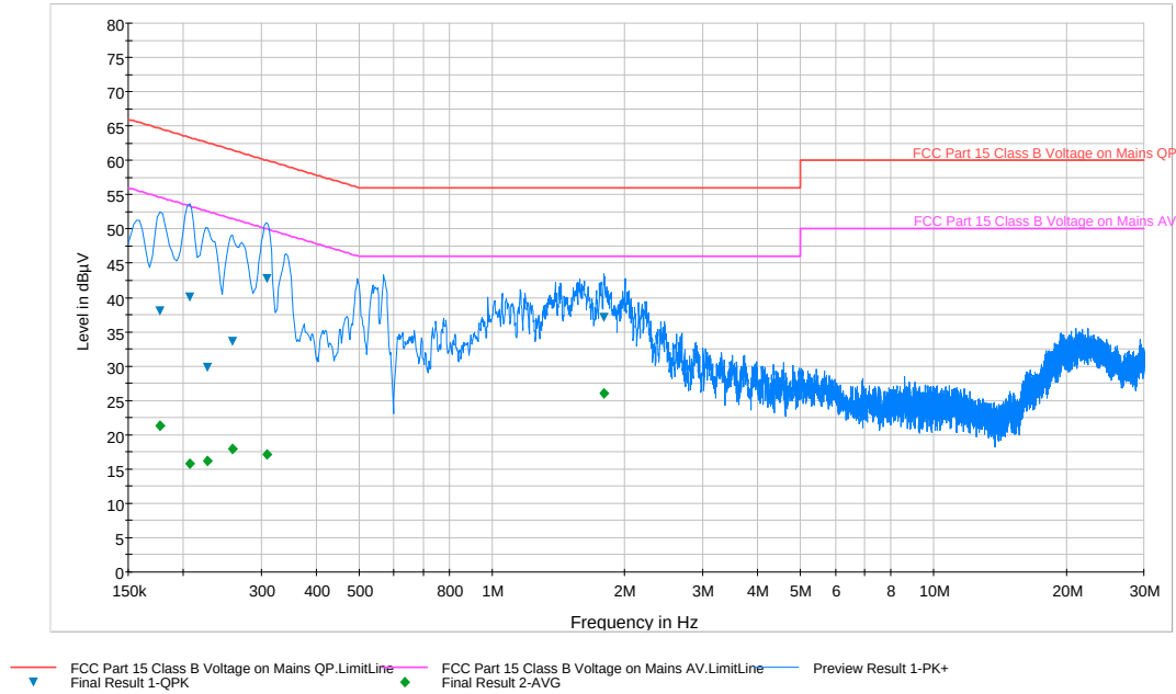
Plot 6-190. Line Conducted Plot with 802.11a UNII Band 1 (N)
