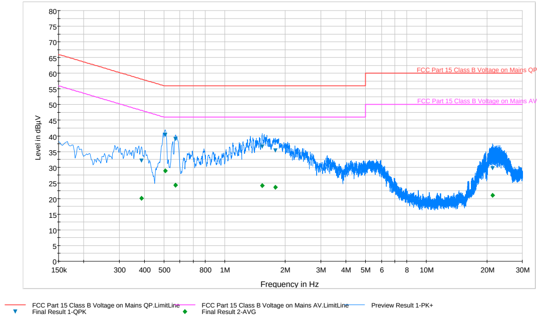
Plot 6-191. Line Conducted Plot with 802.11a UNII Band 2A (L1)
