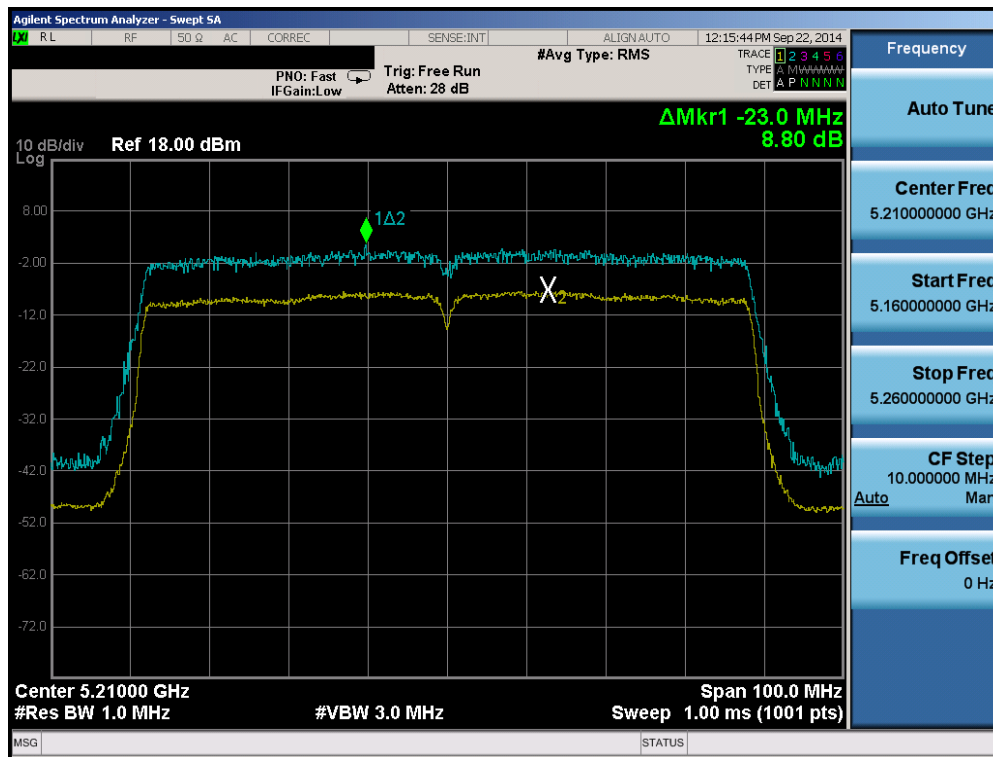
Plot 6-121. Peak Excursion Ratio Plot (80MHz BW 802.11ac (UNII Band 1) – Ch. 42)
