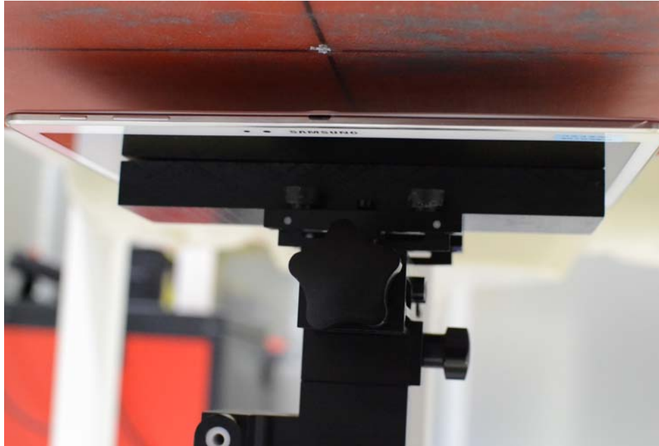
SAR Test Setup Photo 1: Back Side at 2.0 cm
