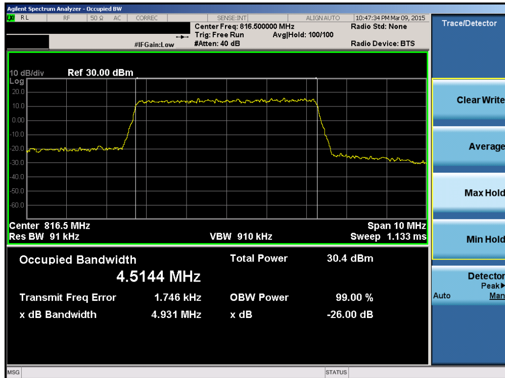
Plot 7-12. Occupied Bandwidth Plot (5MHz QPSK – RB Size 25– Low Channel)
