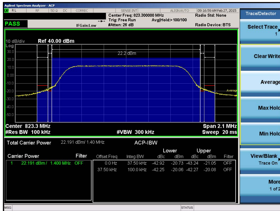
Plot 7-4. Channel Edge Plot (1.4MHz QPSK – RB Size 6 – High Channel)
