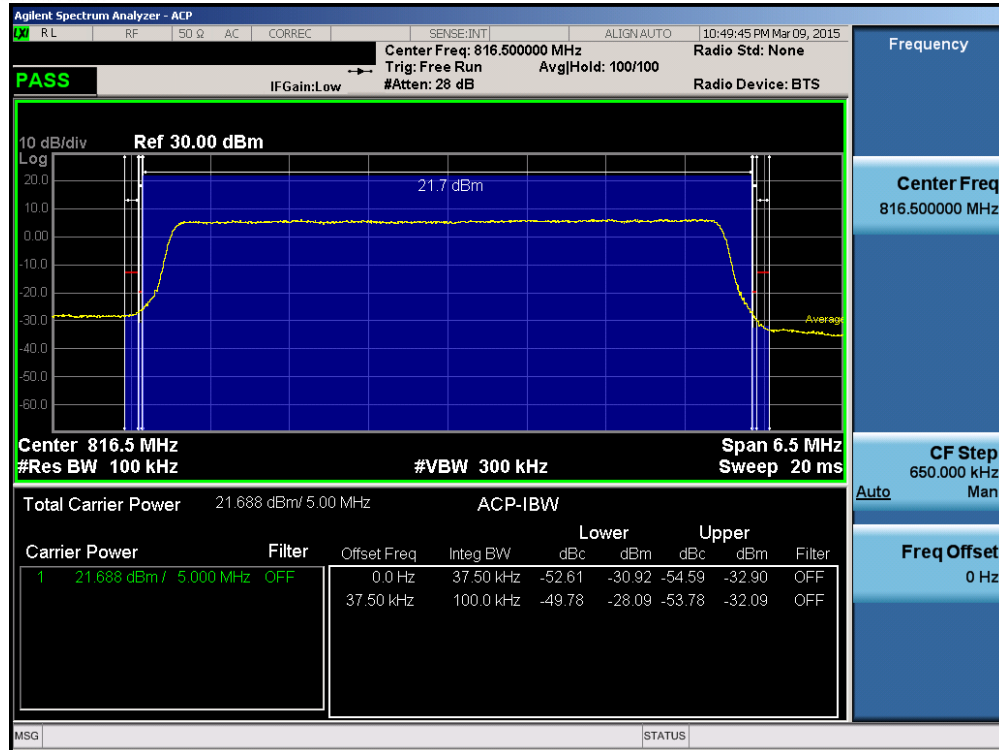
Plot 7-11. Channel Edge Plot (5MHz QPSK – RB Size 25– Low Channel)
