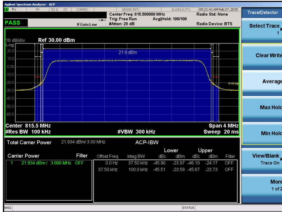
Plot 7-5. Channel Edge Plot (3.0MHz QPSK - RB Size 15- Low Channel)
