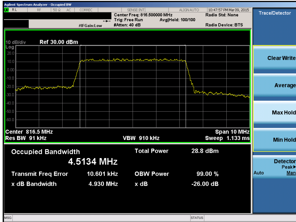
Plot 7-13. Occupied Bandwidth Plot (5MHz 16-QAM – RB Size 25– Low Channel)
