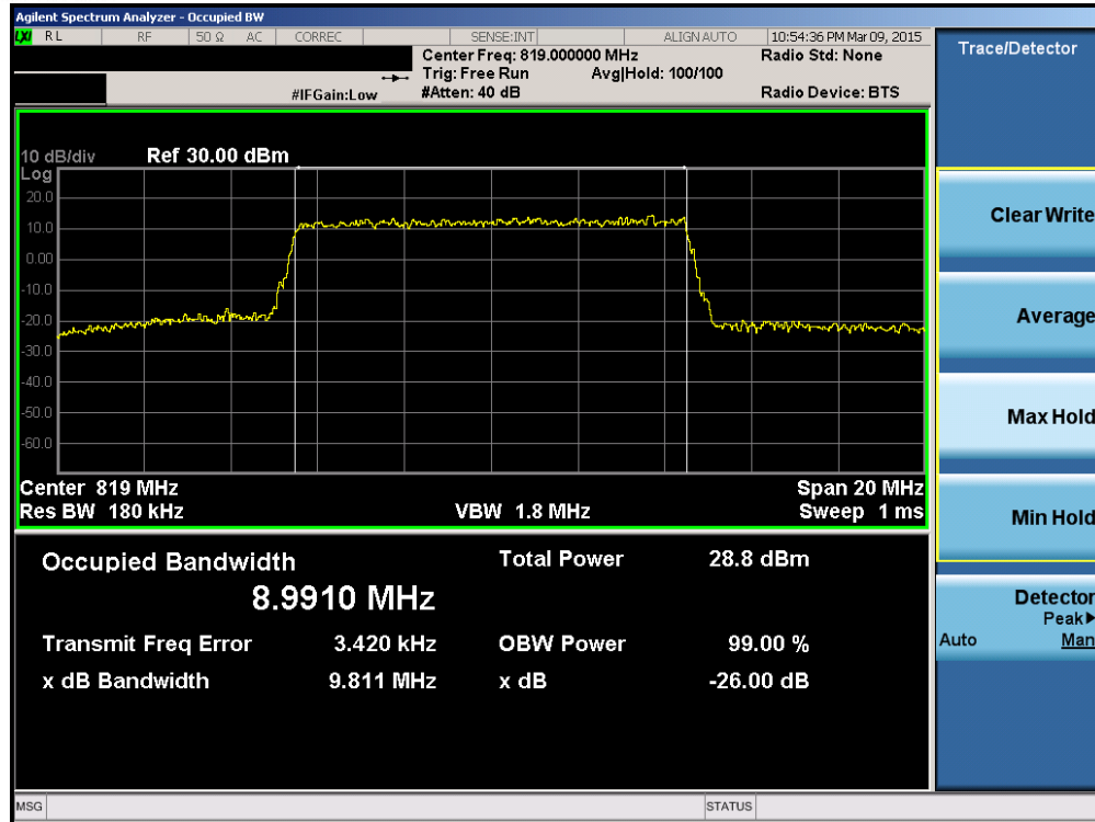
Plot 7-19. Occupied Bandwidth Plot (10MHz 16-QAM – RB Size 50 – Low Channel)
