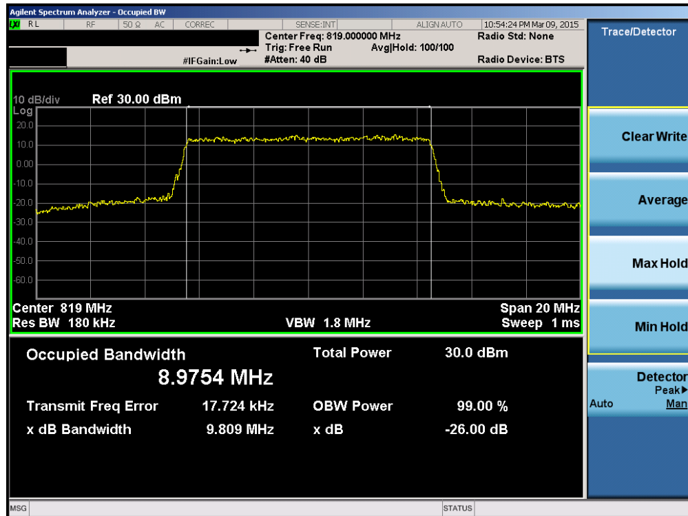
Plot 7-18. Occupied Bandwidth Plot (10MHz QPSK – RB Size 50 – Low Channel)
