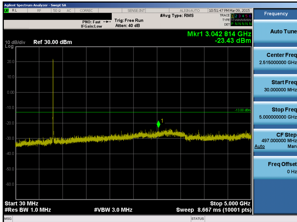
Plot 7-14. Conducted Spurious Plot (5MHz QPSK – RB 1, RB Offset 0 – High Channel)
