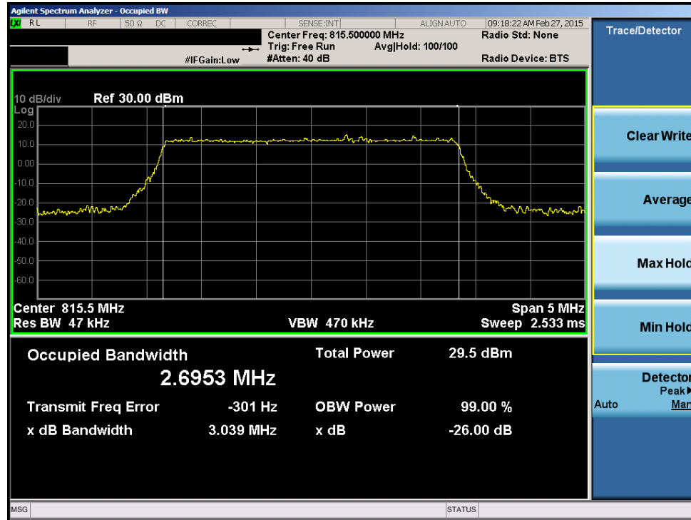
Plot 7-7. Occupied Bandwidth Plot (3.0MHz 16-QAM – RB Size 15– Low Channel)
