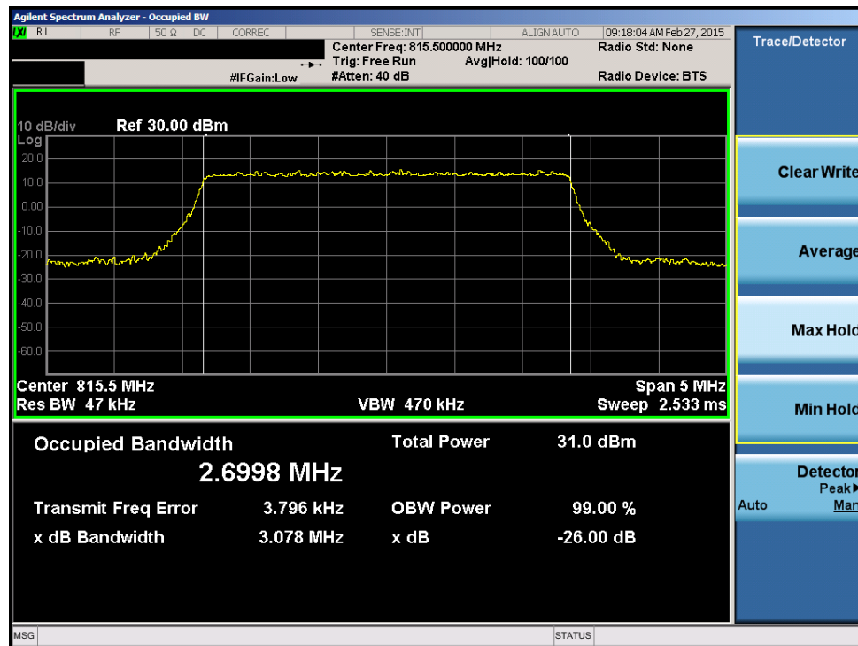
Plot 7-6. Occupied Bandwidth Plot (3.0MHz QPSK - RB Size 15- Low Channel)
