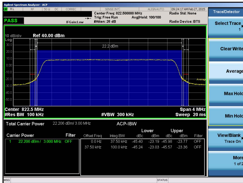
Plot 7-8. Channel Edge Plot (3.0MHz QPSK – RB Size 15 – High Channel)
