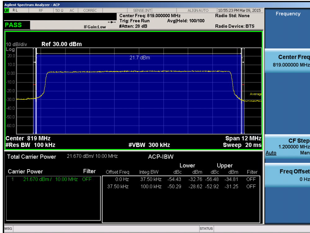
Plot 7-17. Channel Edge Plot (10MHz QPSK – RB Size 50 – Low Channel)
