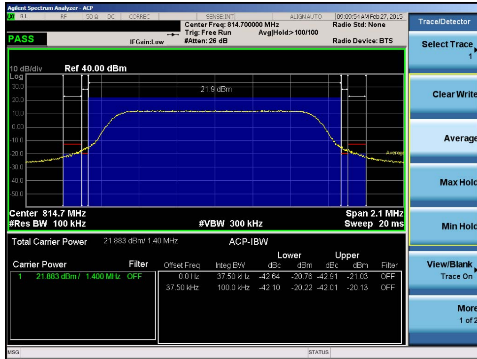
Plot 7-1. Channel Edge Plot (1.4MHz QPSK – RB Size 6– Low Channel)
